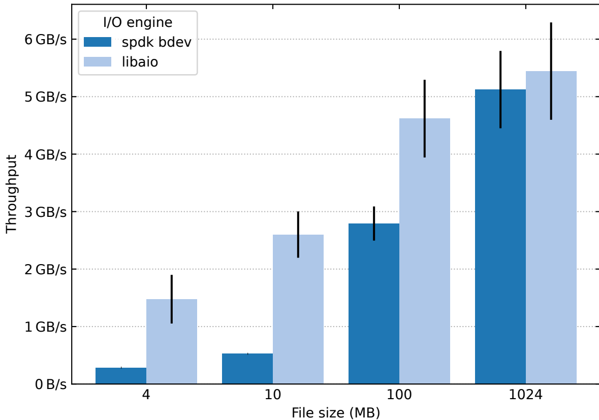
Sequential write throughput with 1MB block size
