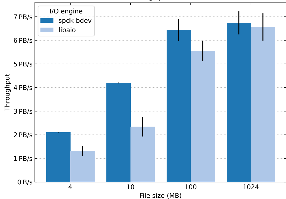
Random read throughput with 4kB block size
