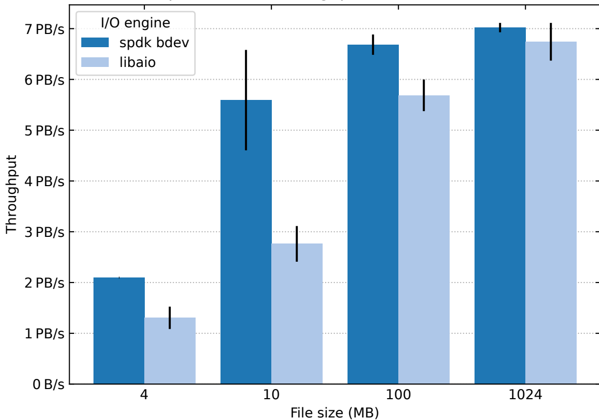
Sequential read throughput with 4kB block size
