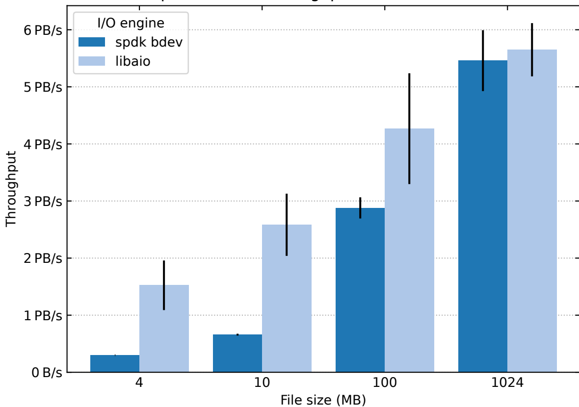
Sequential write throughput with 4kB block size
