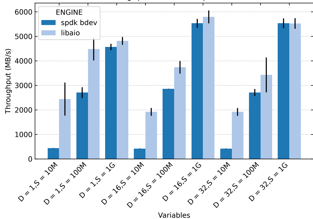
Randw throughput (D = I/O Depth, S = file size)
