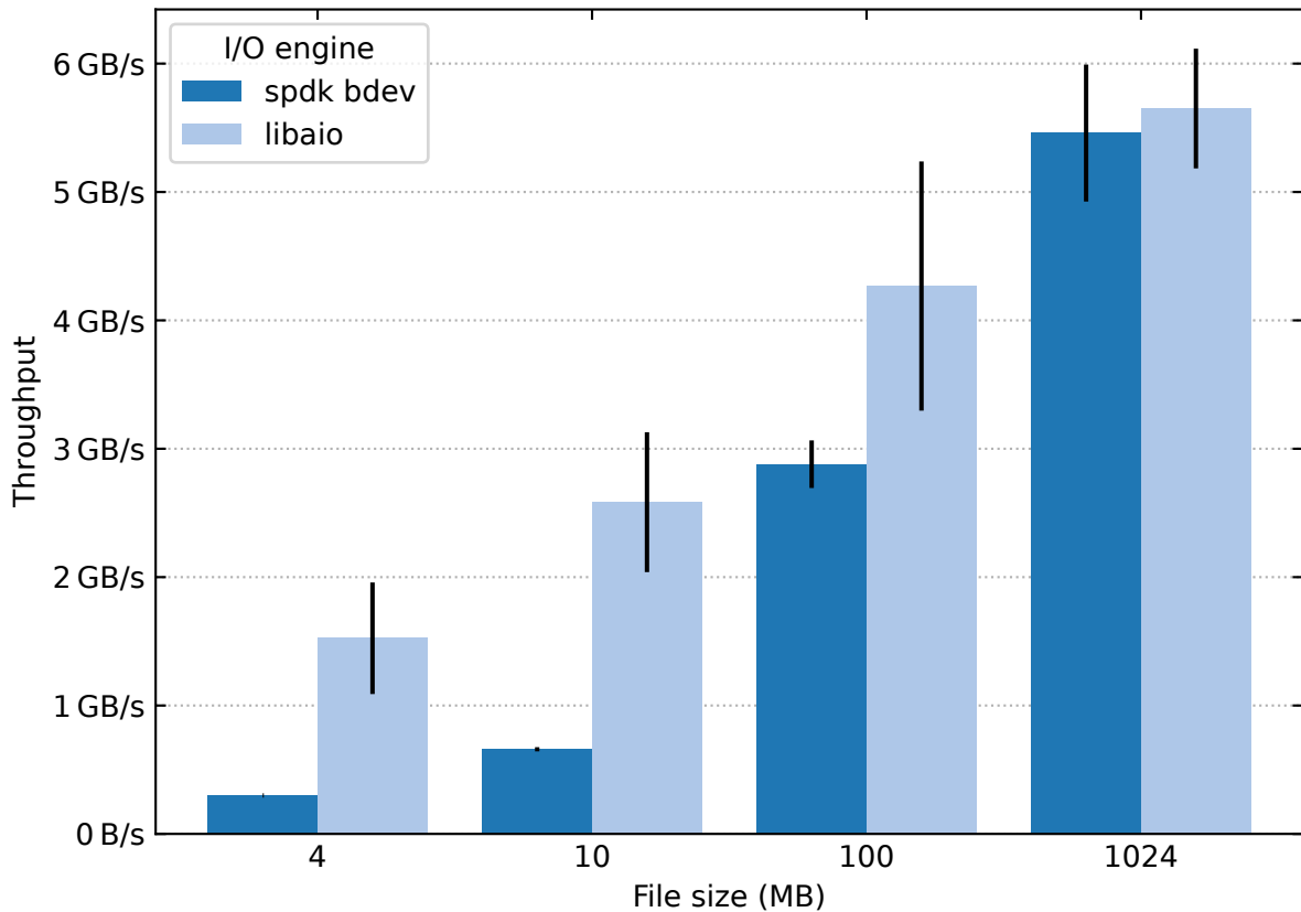
Sequential write throughput with 4MB block size
