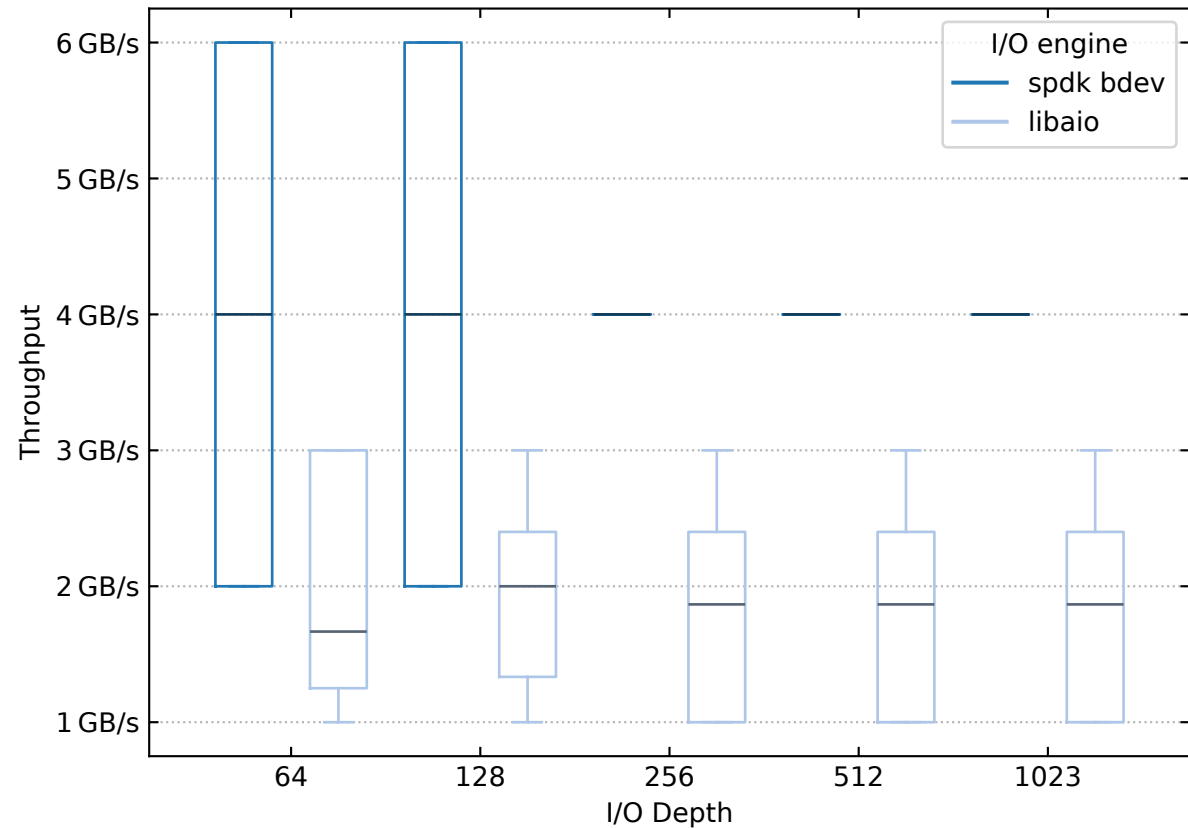
Sequential read throughput with variables I/O depth
