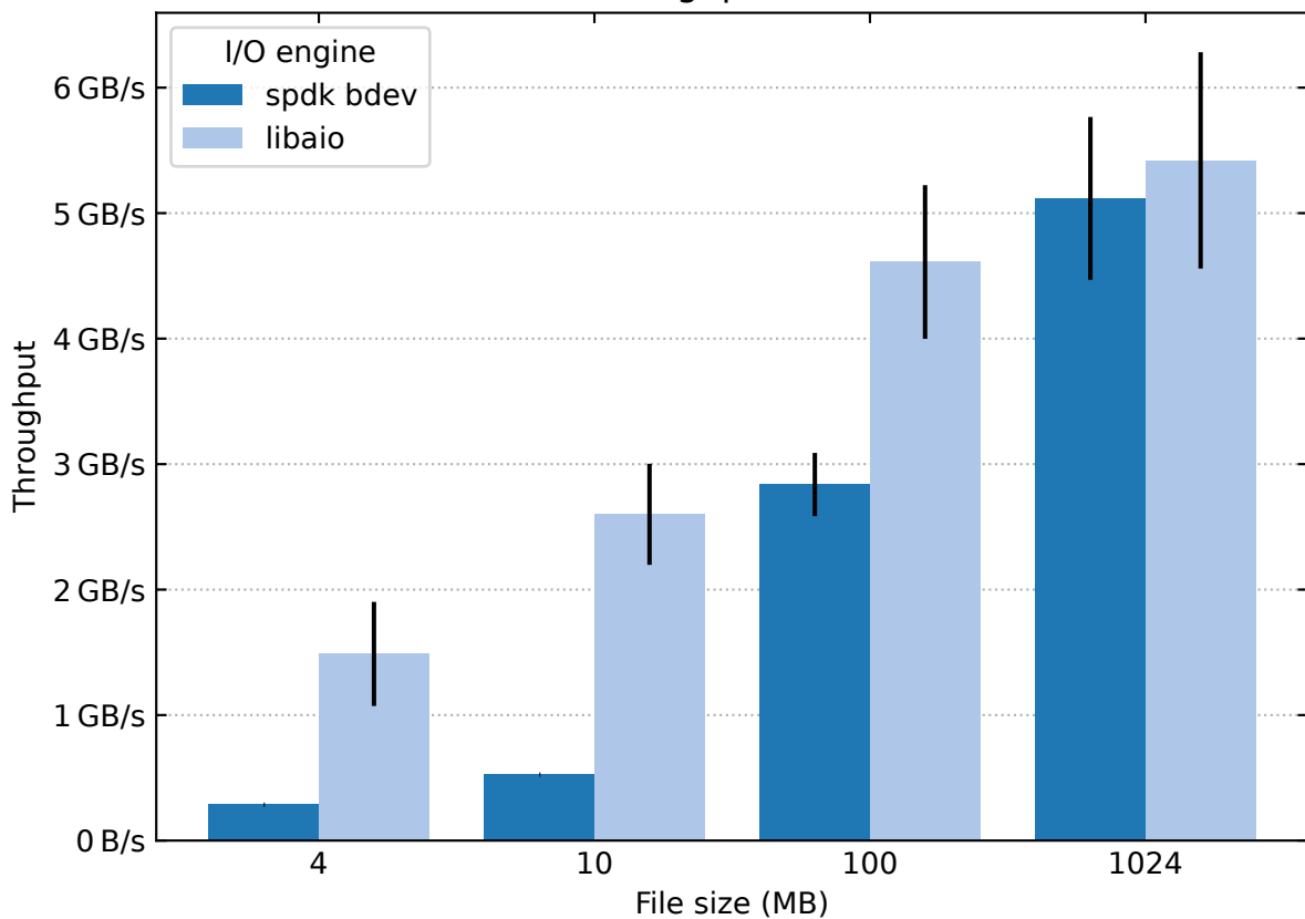
Random write throughput with 1MB block size
