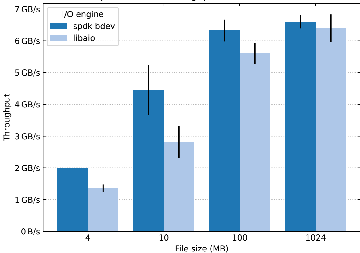
Sequential read throughput with 1MB block size
