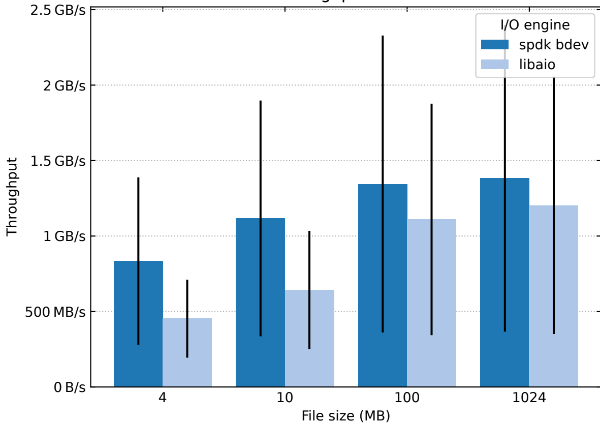
Random read throughput with 4kB block size
