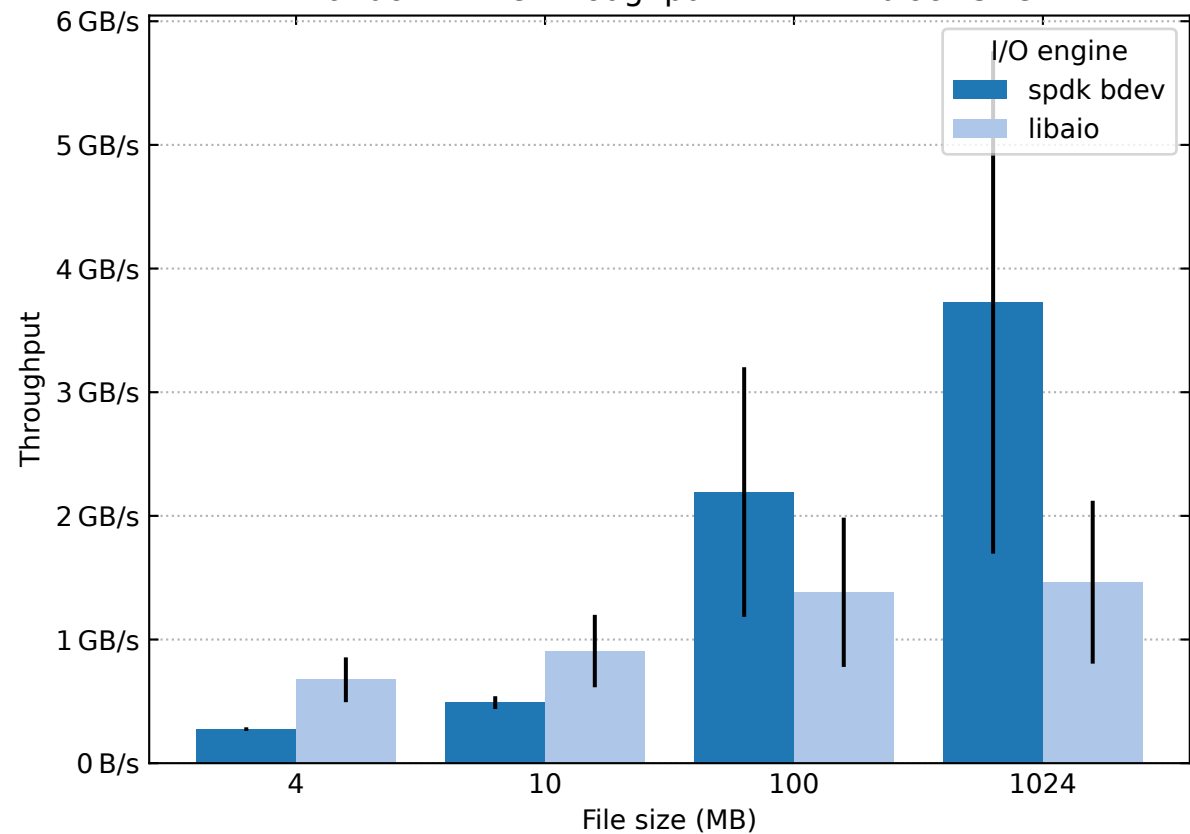
Random write throughput with 4kB block size
