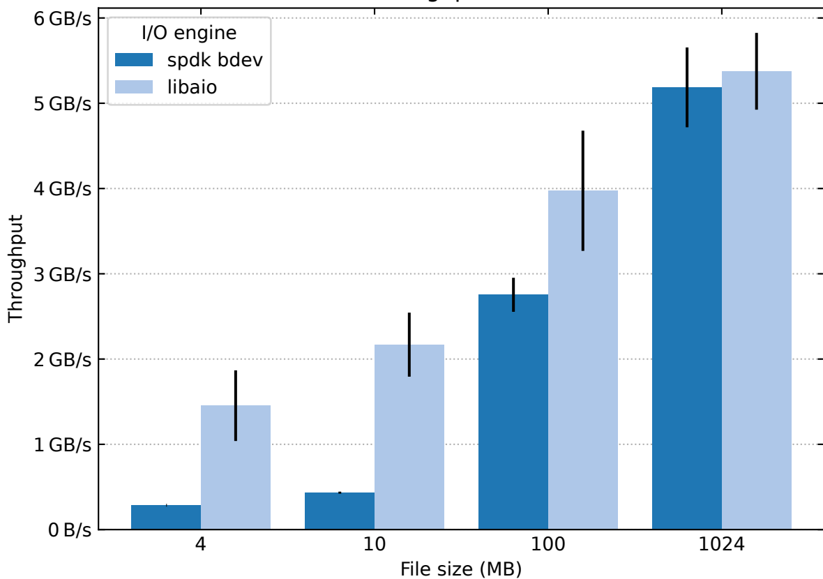
Random write throughput with 4MB block size
