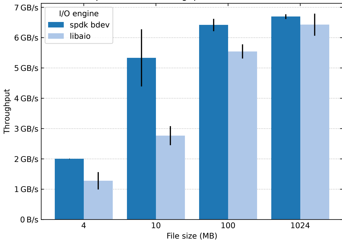
Sequential read throughput with 4MB block size
