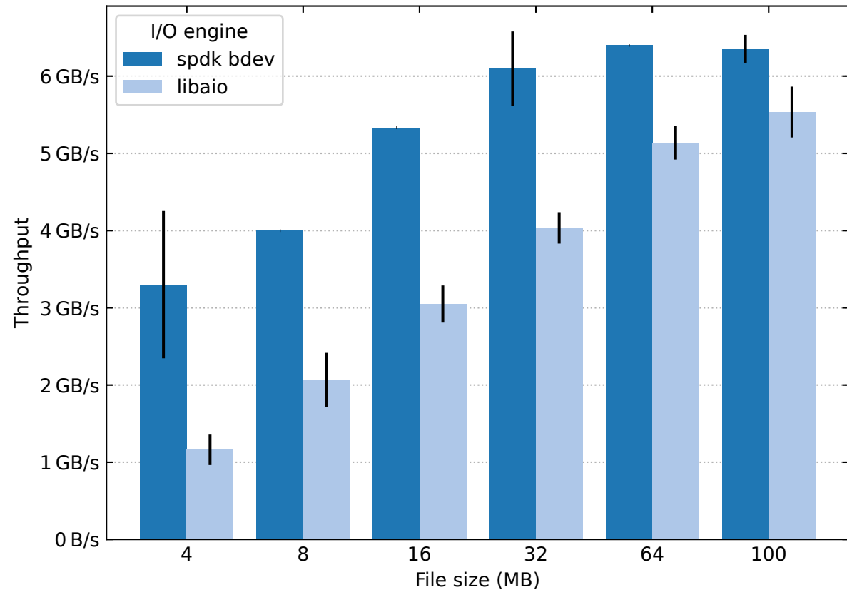
Sequential read throughput with aggregated I/O depth
