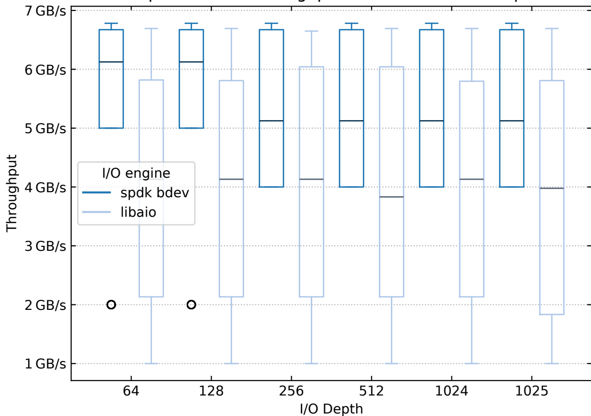
Sequential read throughput with variables I/O depth
