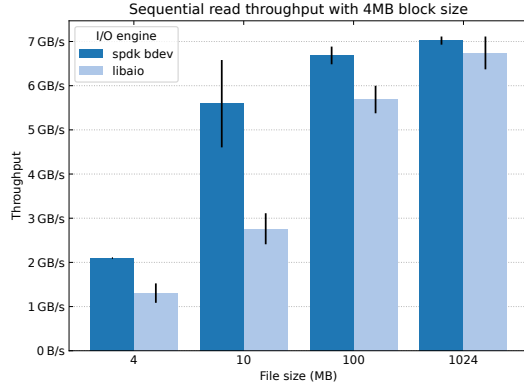
Figure 3.1: Throughput of sequential read operations with 4MB block size
