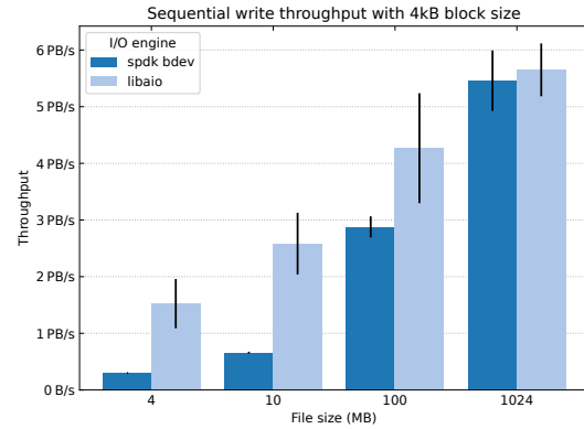
Figure 3.4: Throughput of sequential write operations with 4kB block size
