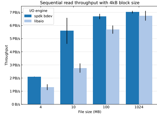
Figure 3.2: Throughput of sequential read operations with 4kB block size
