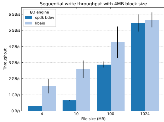
Figure 3.3: Throughput of sequential write operations with 4MB block size
