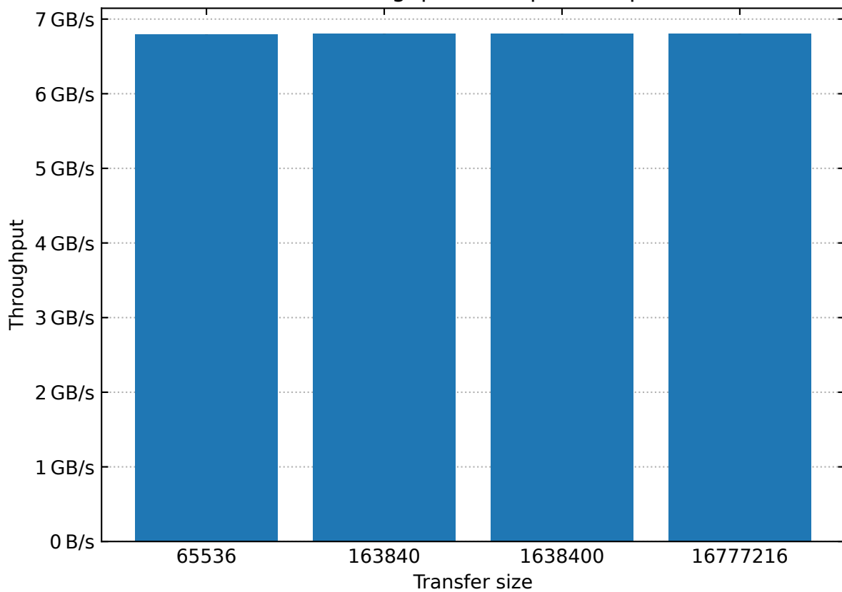
Random read throughput with queue depth set to 64
