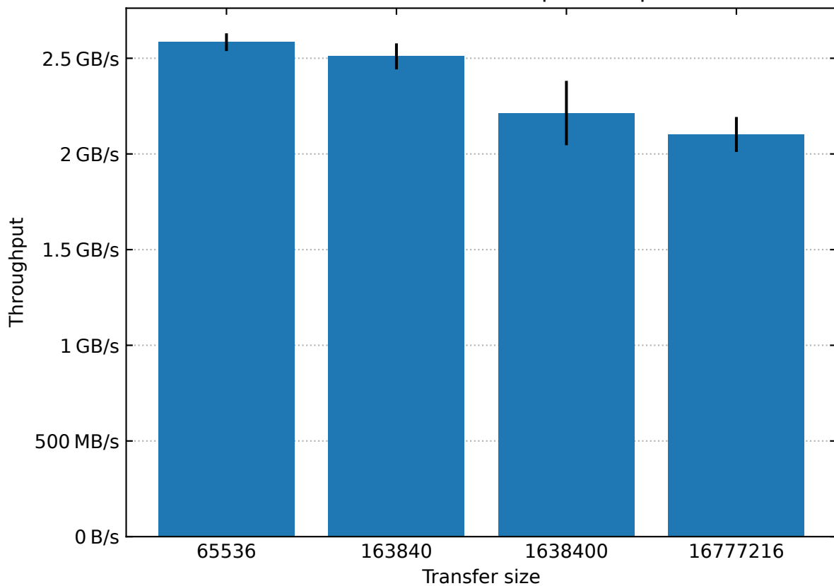
Random mixed read/write with queue depth set to 64
