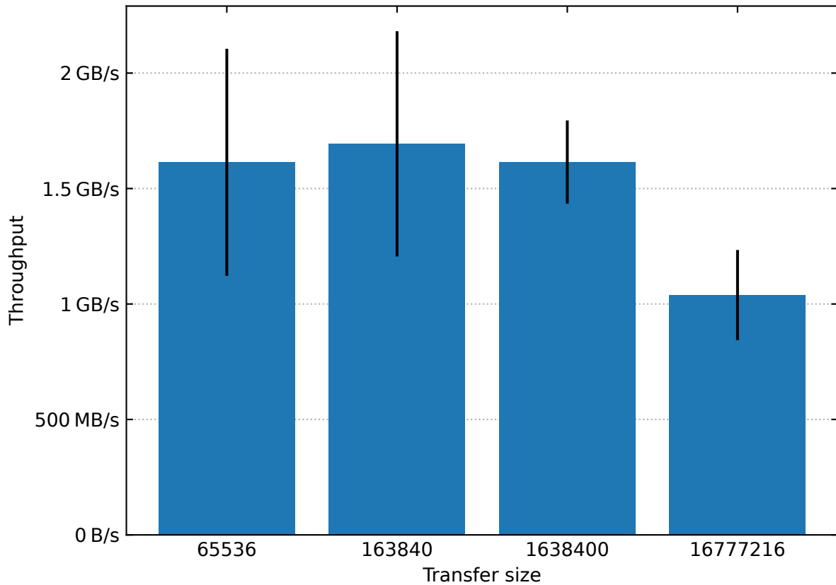
Random write throughput with queue depth set to 64
