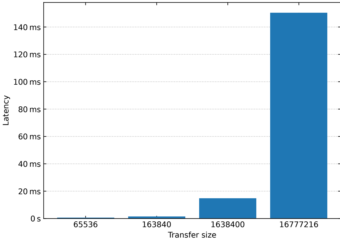
Sequential mixed read/write with queue depth set to 64
