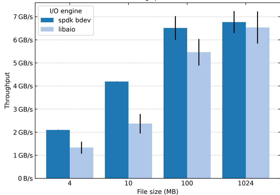
Random read throughput with 4MB block size
