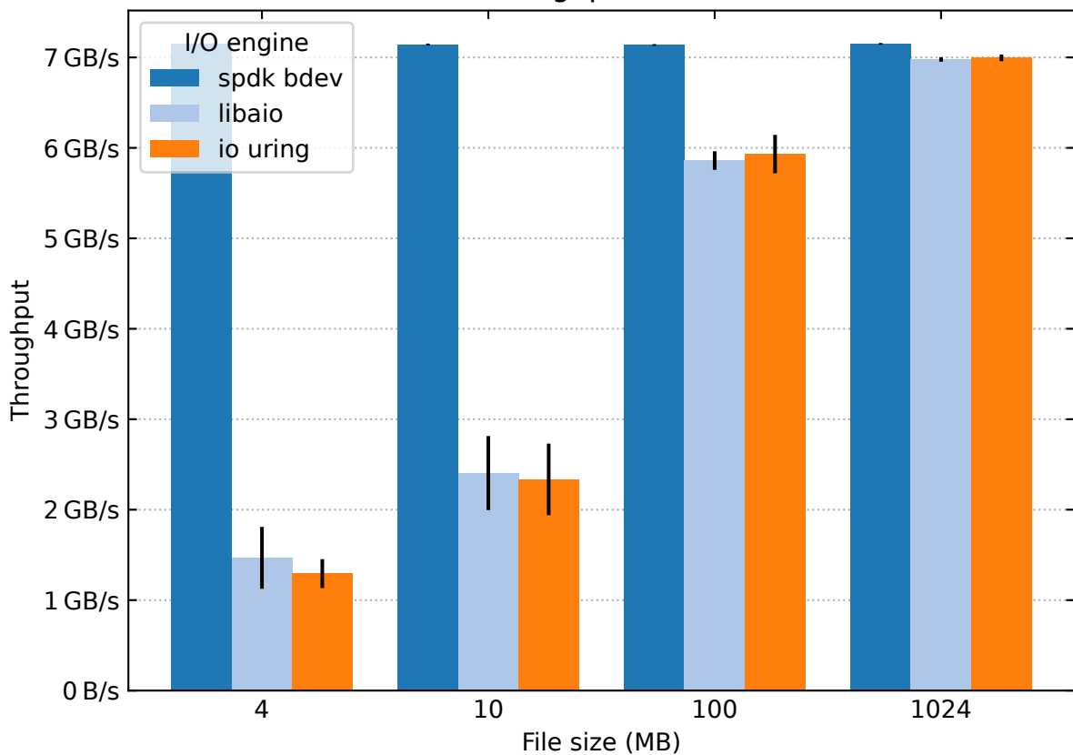
Random read throughput with 4MB block size
