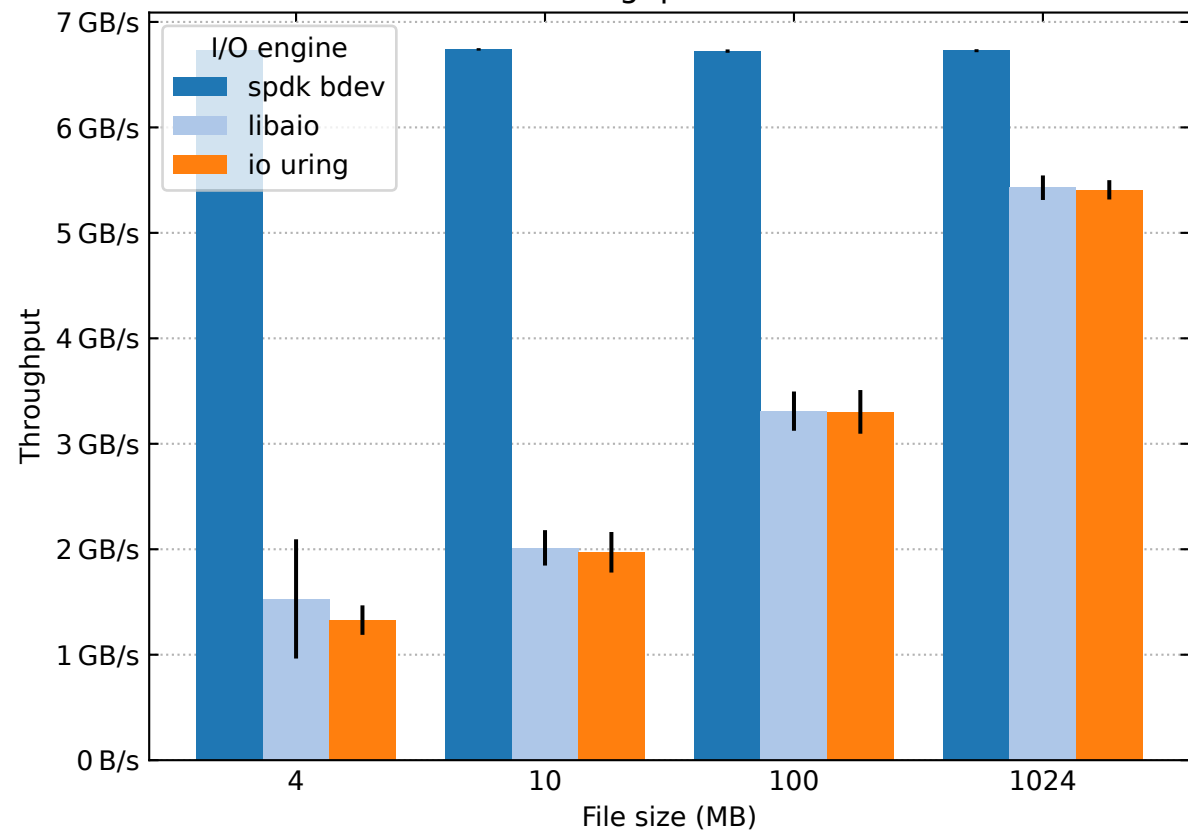
Random write throughput with 4MB block size
