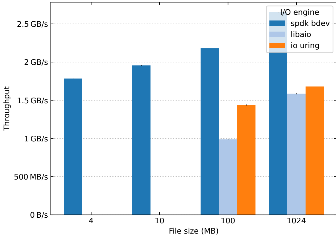
Sequential mixed read/write with 4MB block size
