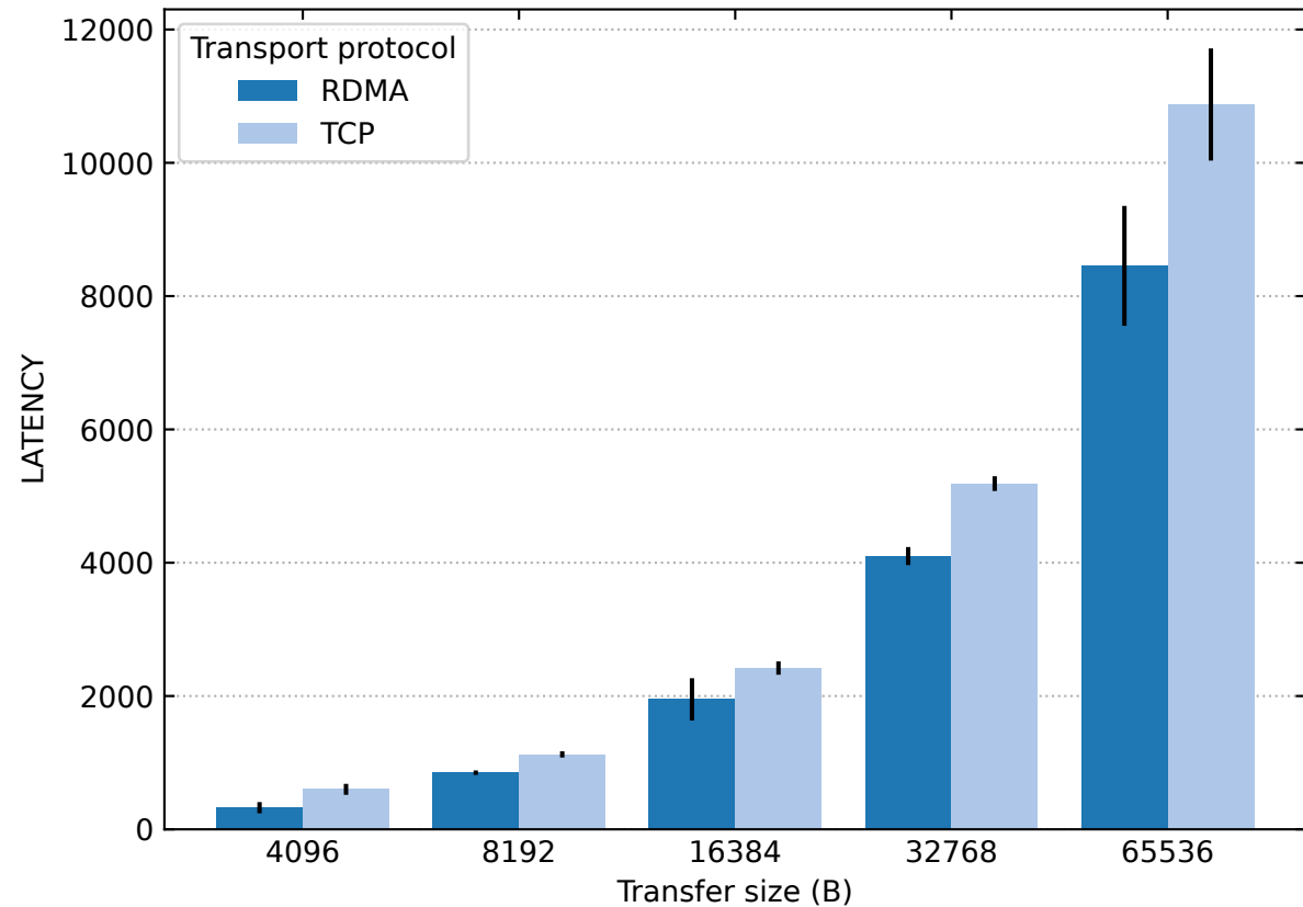
NVMe-oF Random mixed read/write with queue depth set to 64
