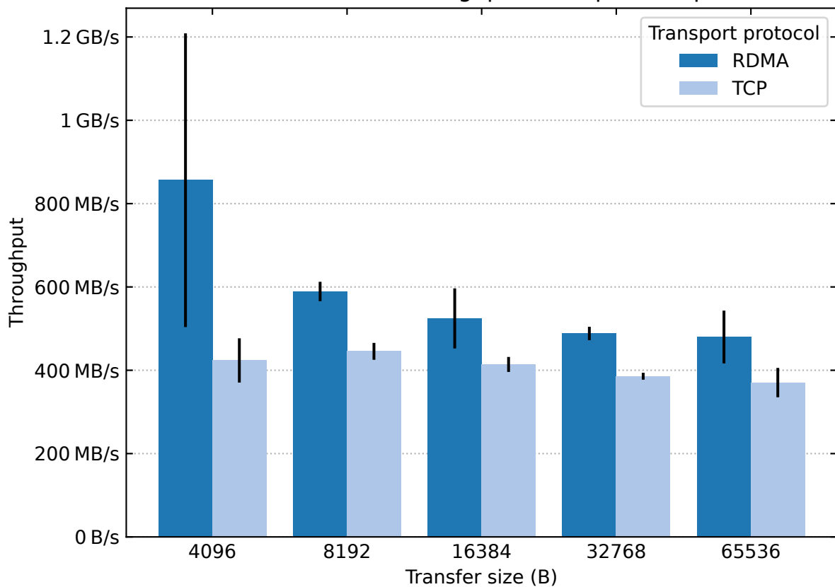
NVMe-oF Random write throughput with queue depth set to 64
