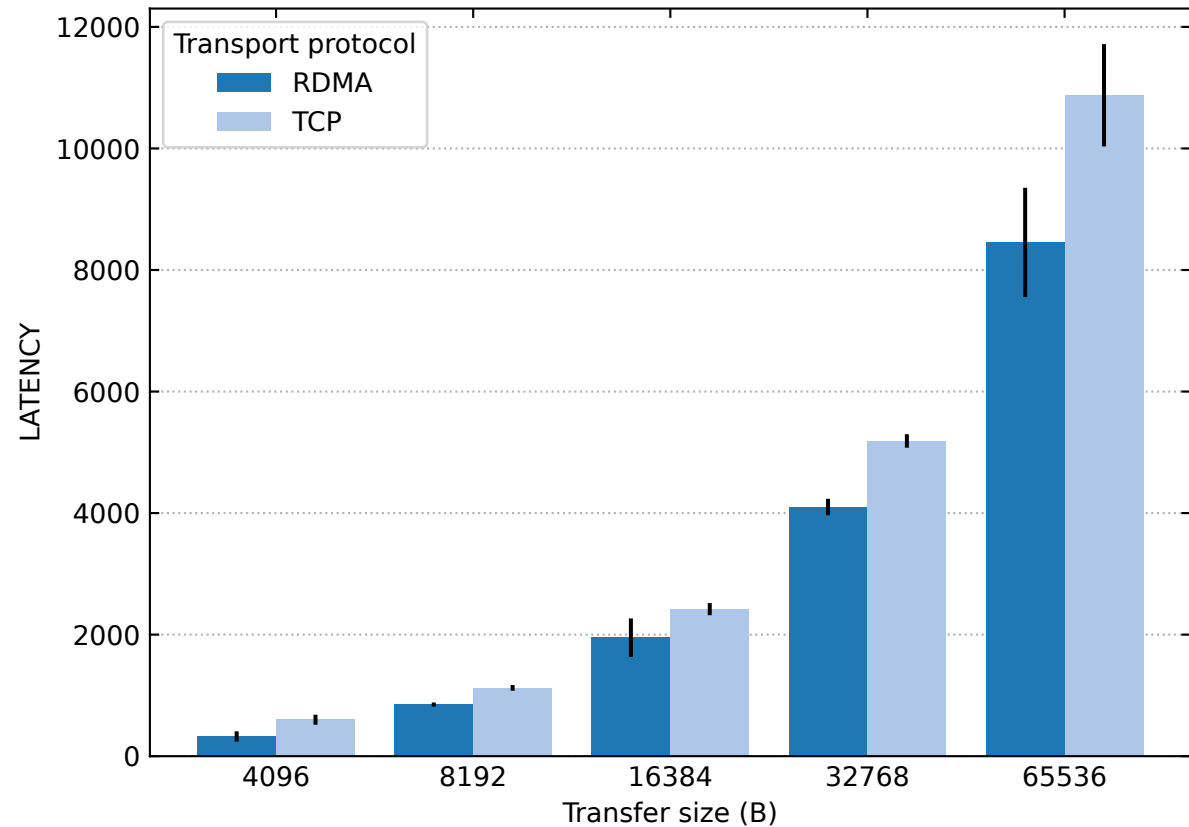
NVMe-oF Sequential mixed read/write with queue depth set to 64
