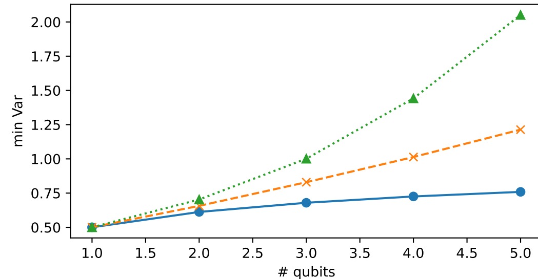
Scaling with number of qubits
