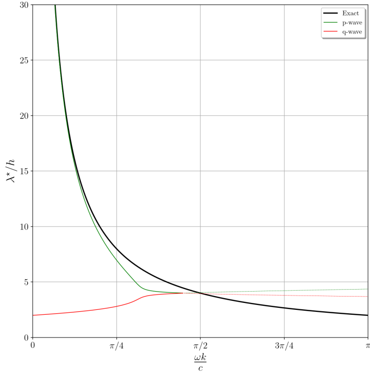
Figure 5: Modified wavelengths of the LW scheme depending on the pulsation \omega . Black line: exact. Green line: p -waves. Red line: q -waves. CFL number is c = 0.1 . Dashed lines are, in this case, evanescent solutions.
