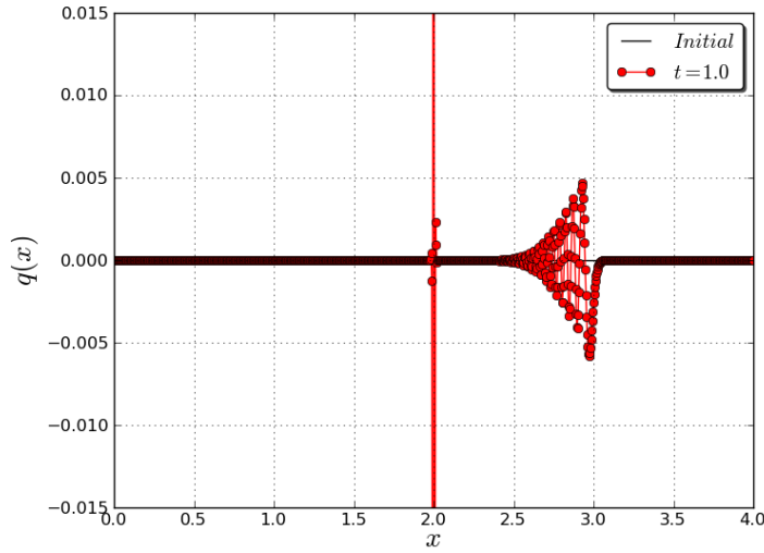
Figure 12: Source term E at x = 2 . Result after 2500 iterations. Black line: Initial solution. Red line: Numerical solution. The scheme is LW and the CFL number is c = 0.1 .
