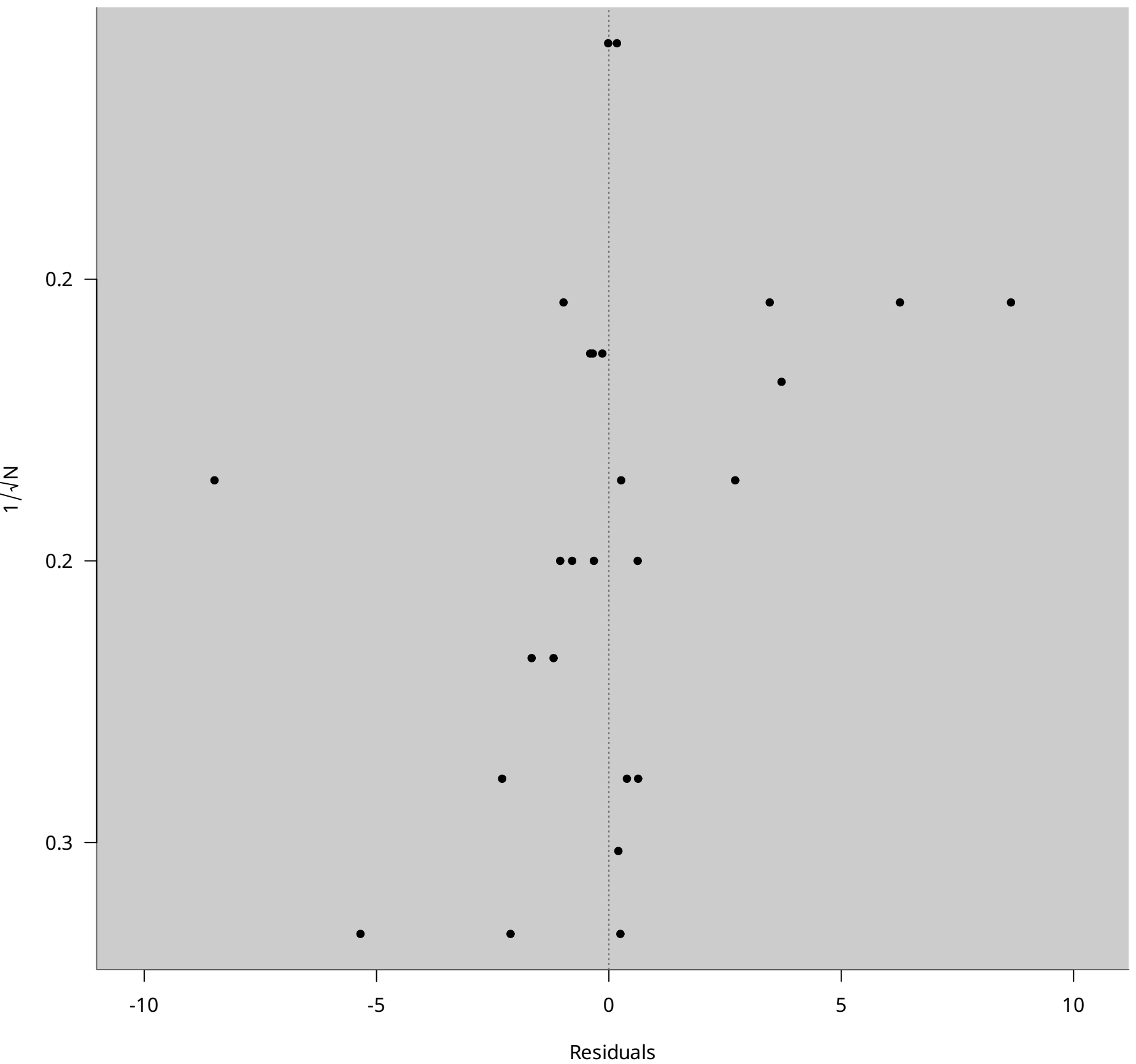
Funnel plot - OFT
