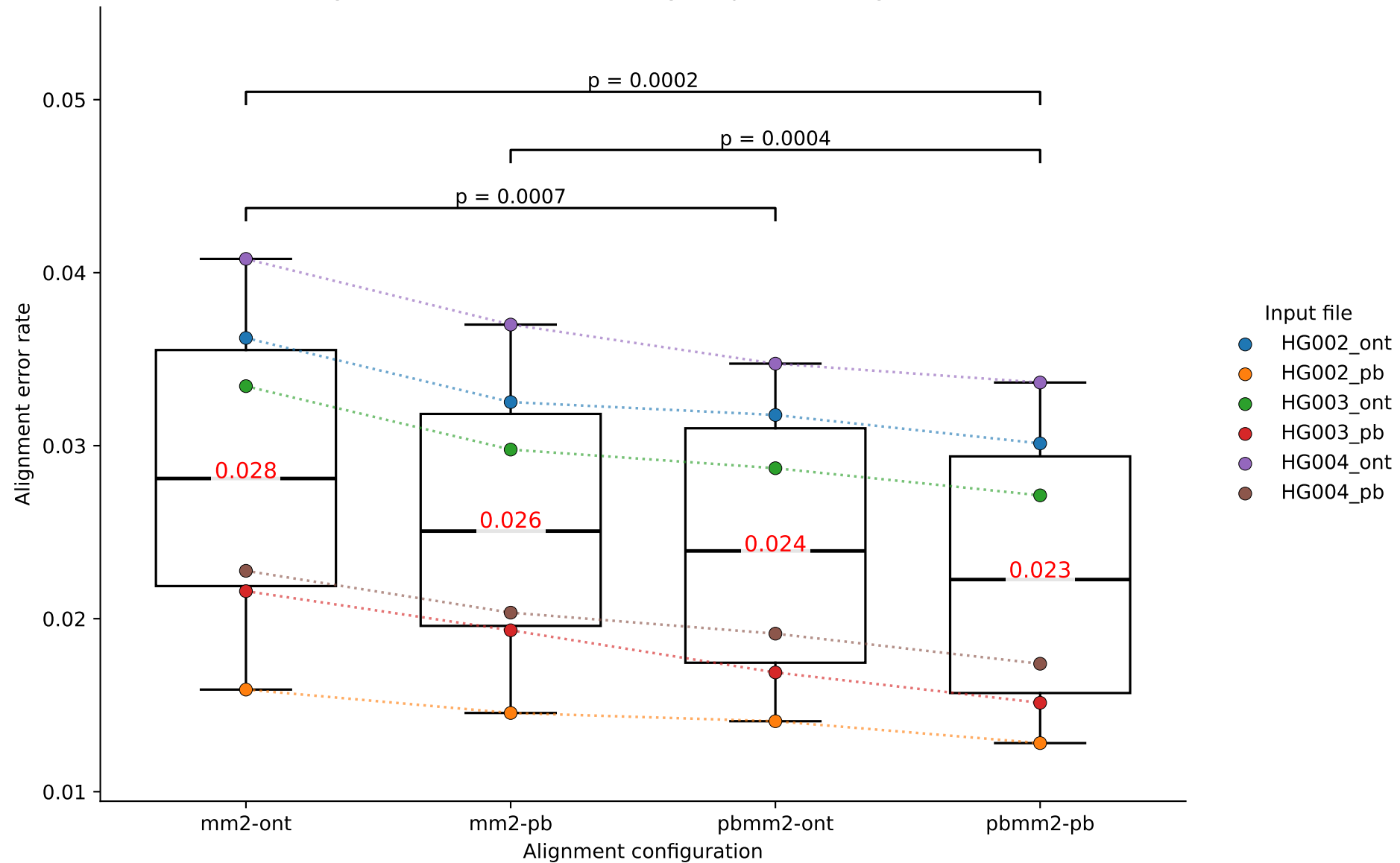
Alignment error rate across aligner-preset configurations
