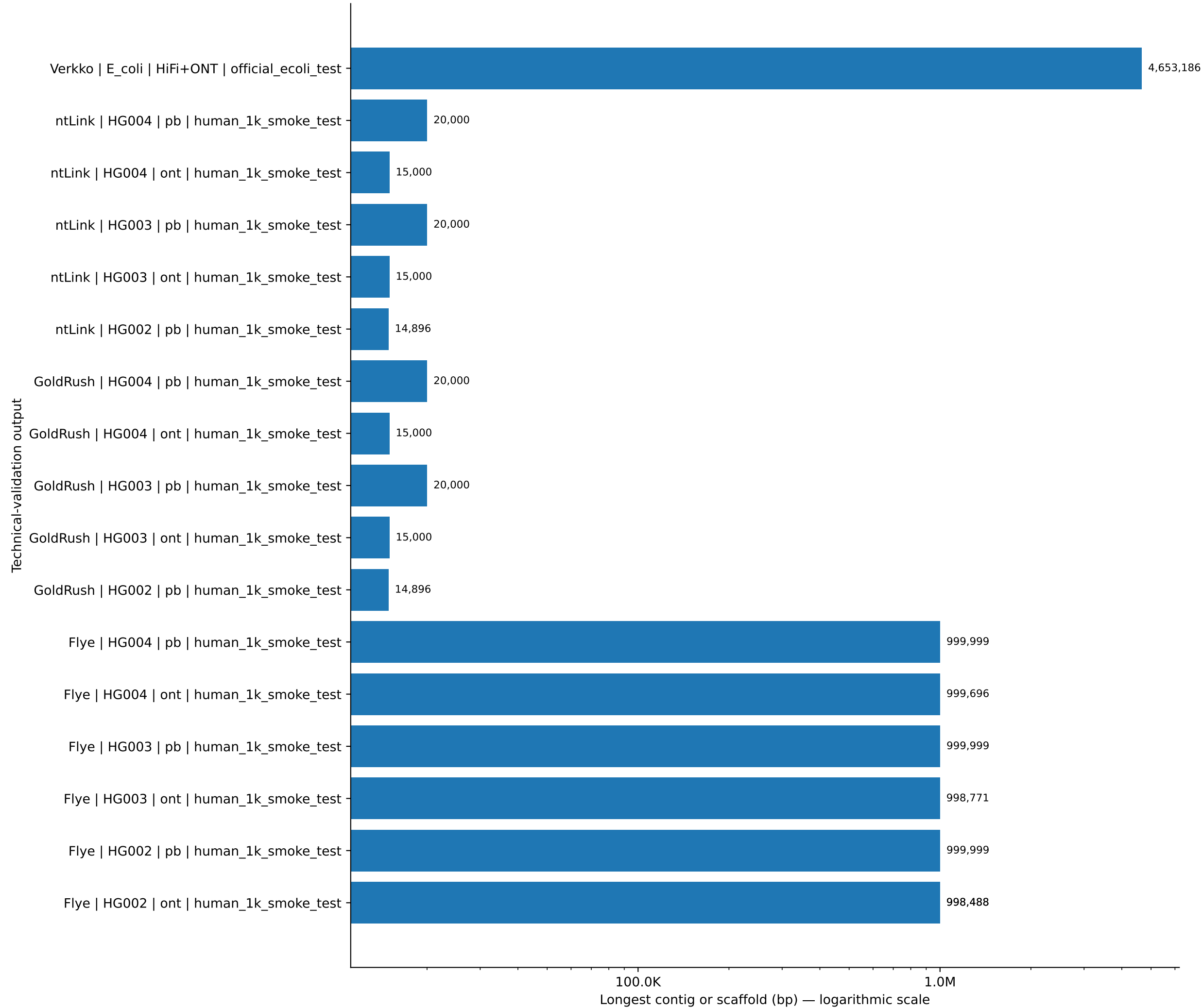
Longest assembled sequence Mixed smoke-test datasets — do not interpret as assembler ranking
