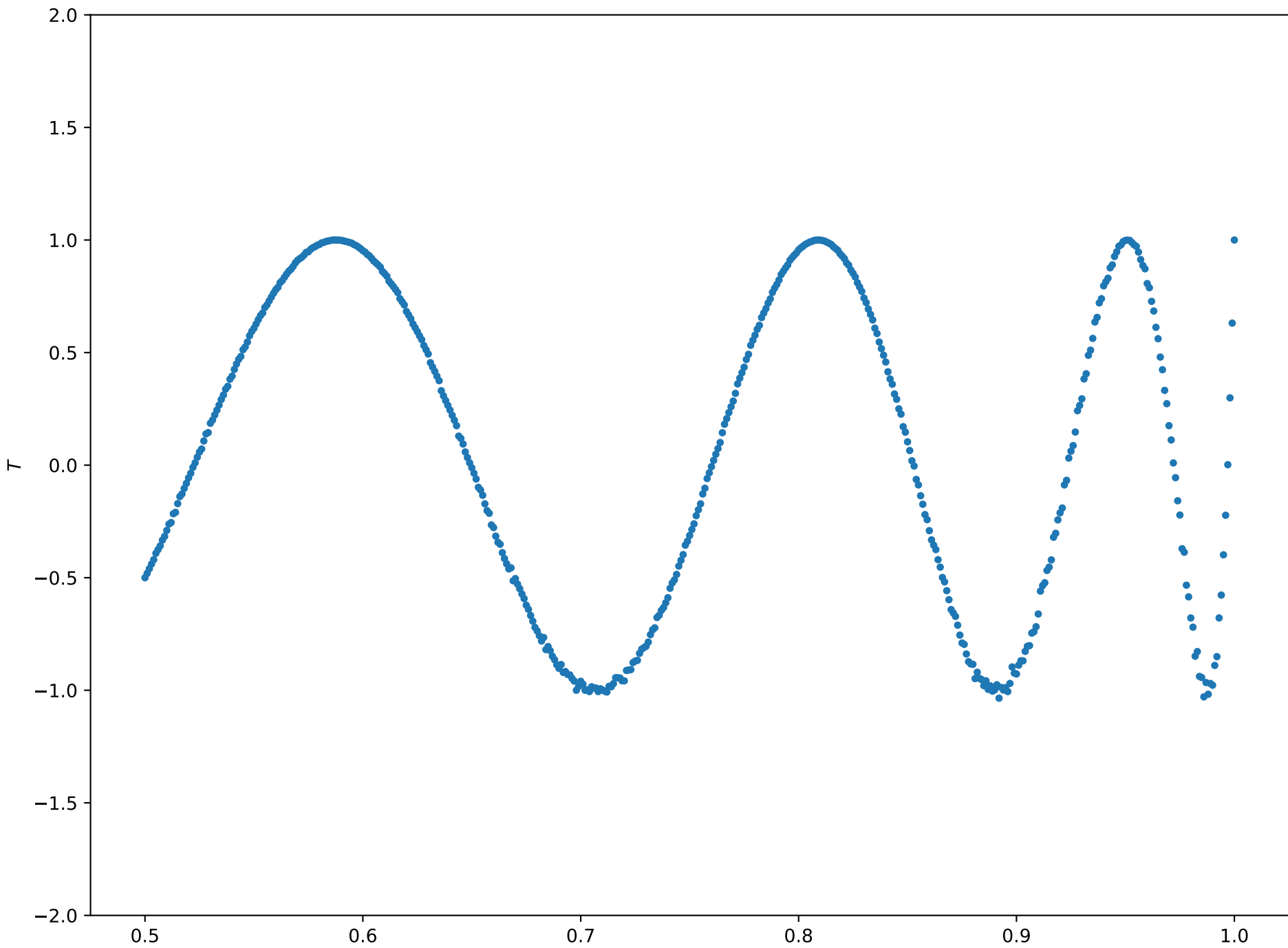
FACTORED-DOUBLE vprec binary16
