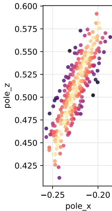
Pole-vector distribution
