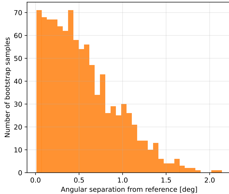
Bootstrap angular uncertainty
