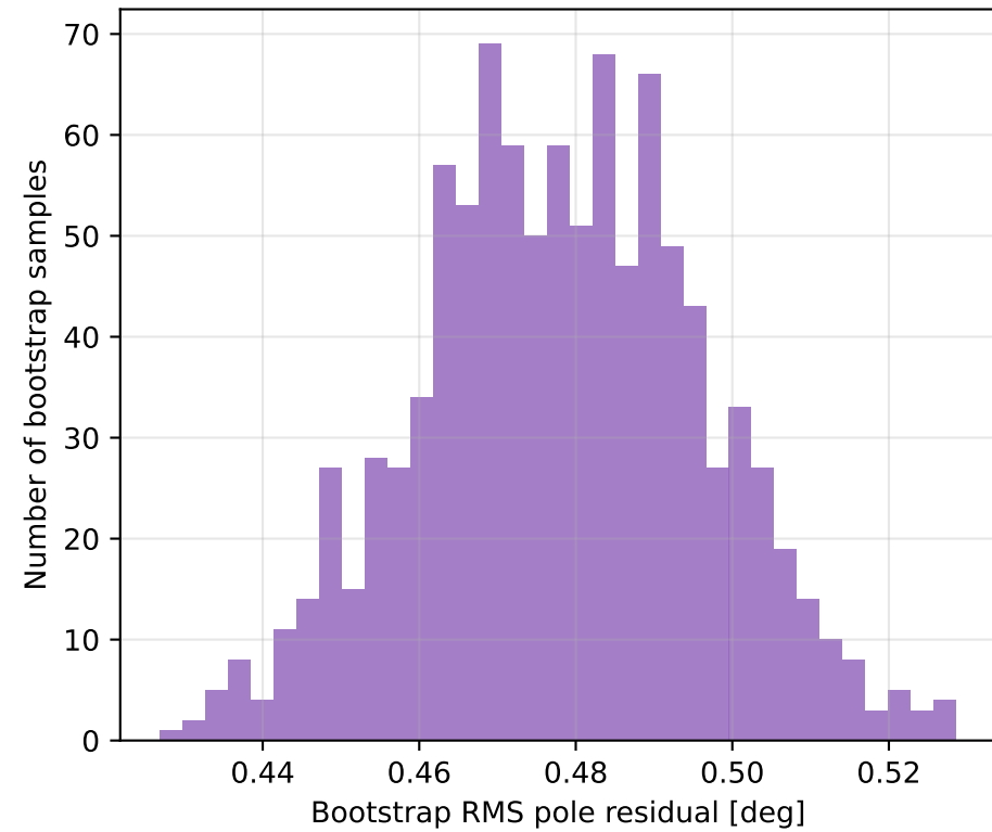
Bootstrap residual stability
