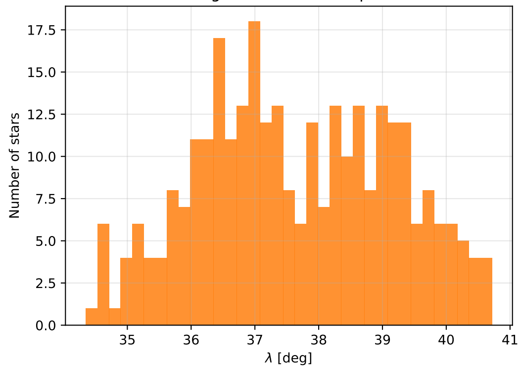
Tangential alignment with apex
