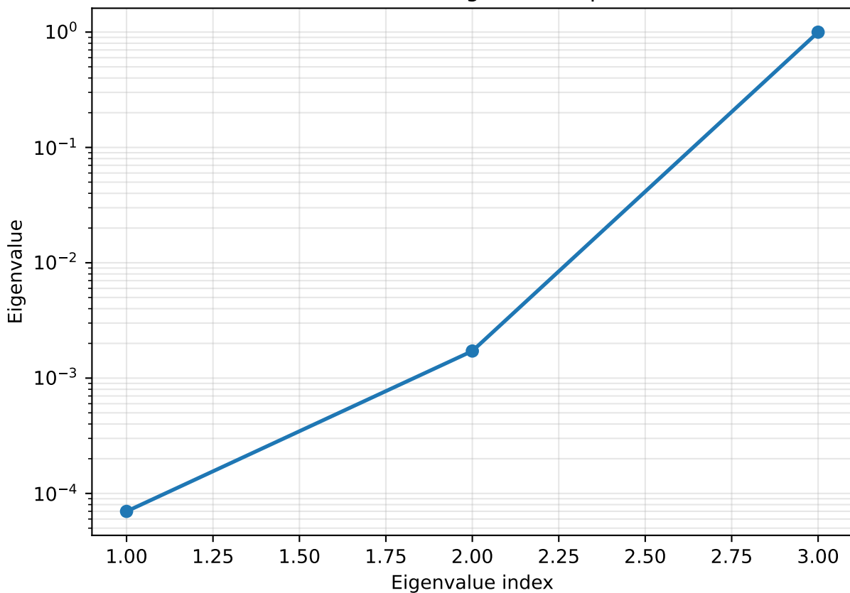
Pole covariance eigenvalue spectrum
