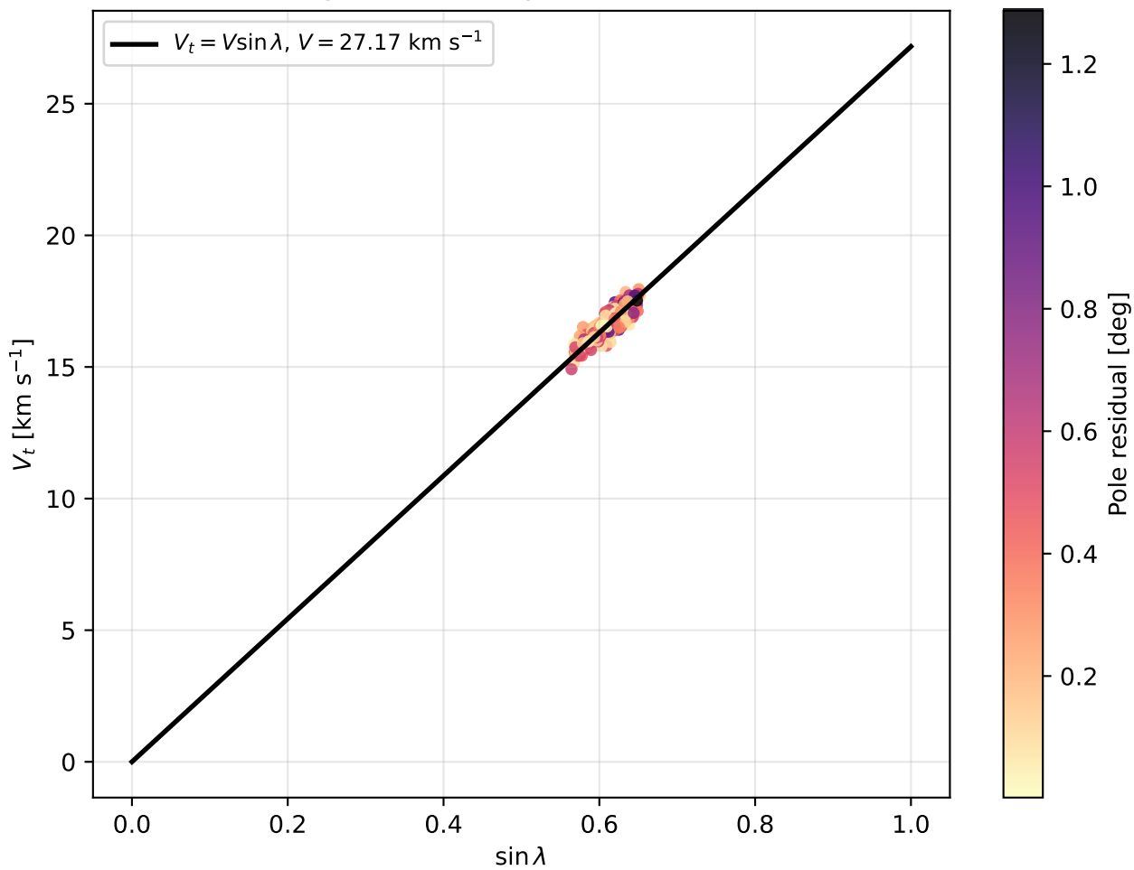
Tangential velocity test: V_t vs. \sin \lambda
