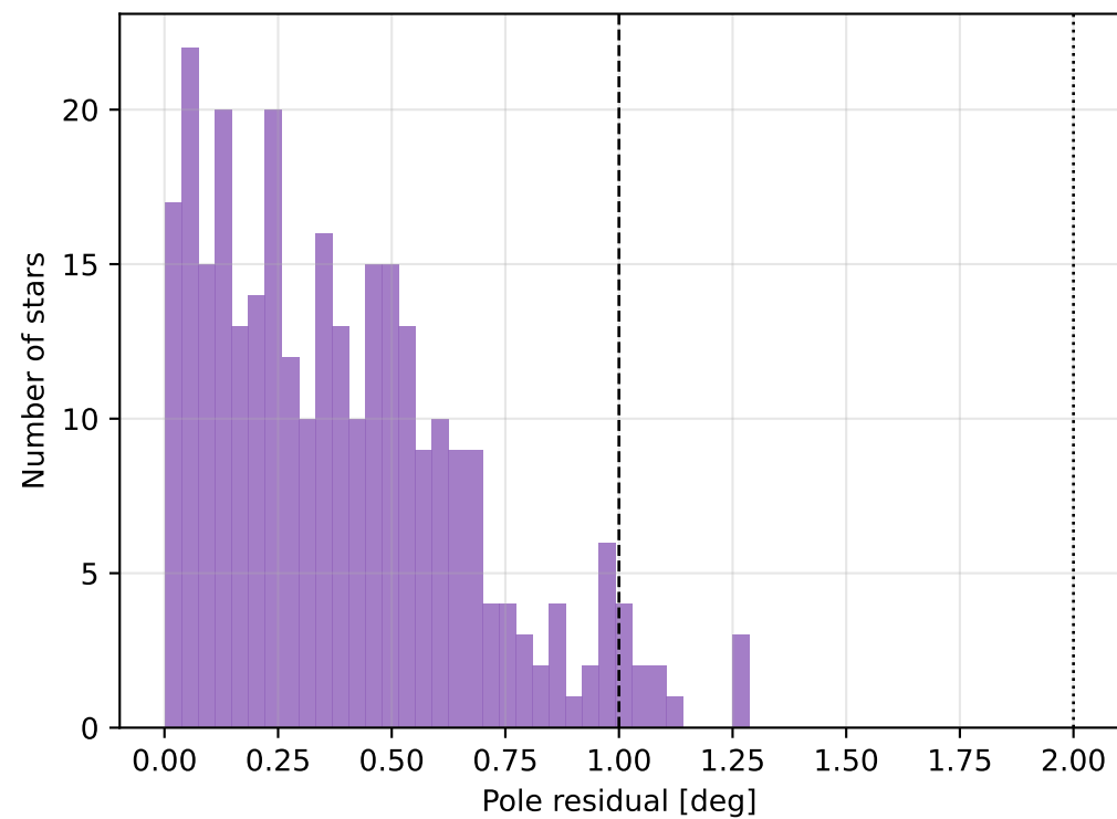
\sin \lambda refinement diagnostic
