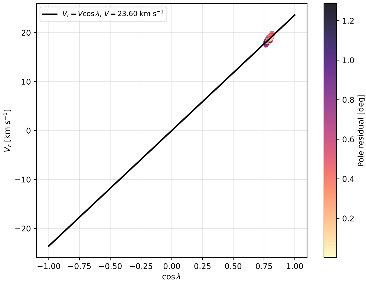
Radial velocity test: V_r vs. \cos \lambda
