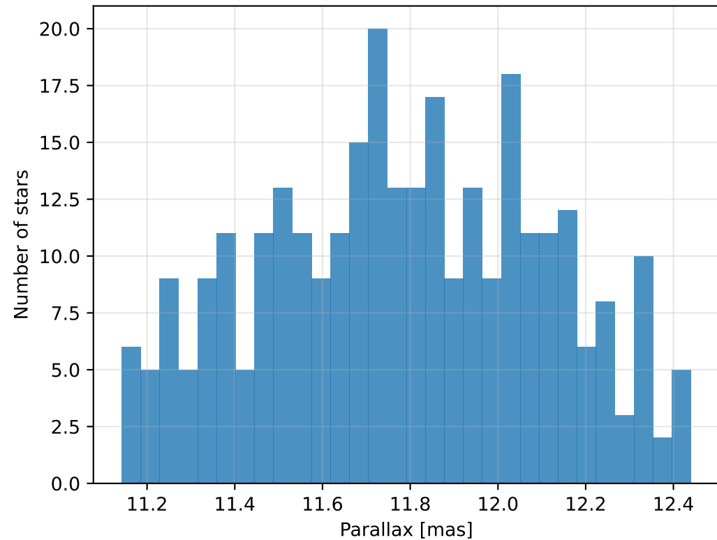
Parallax distribution
