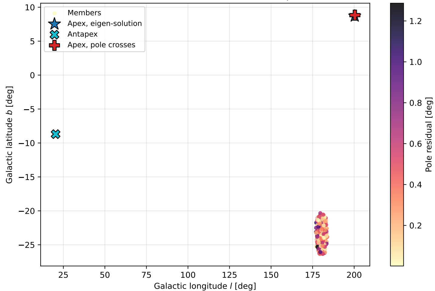
Galactic distribution and recovered apex
