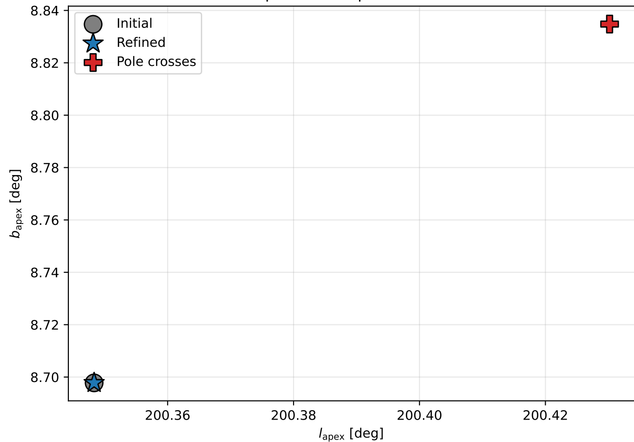
Comparison of apex estimators
