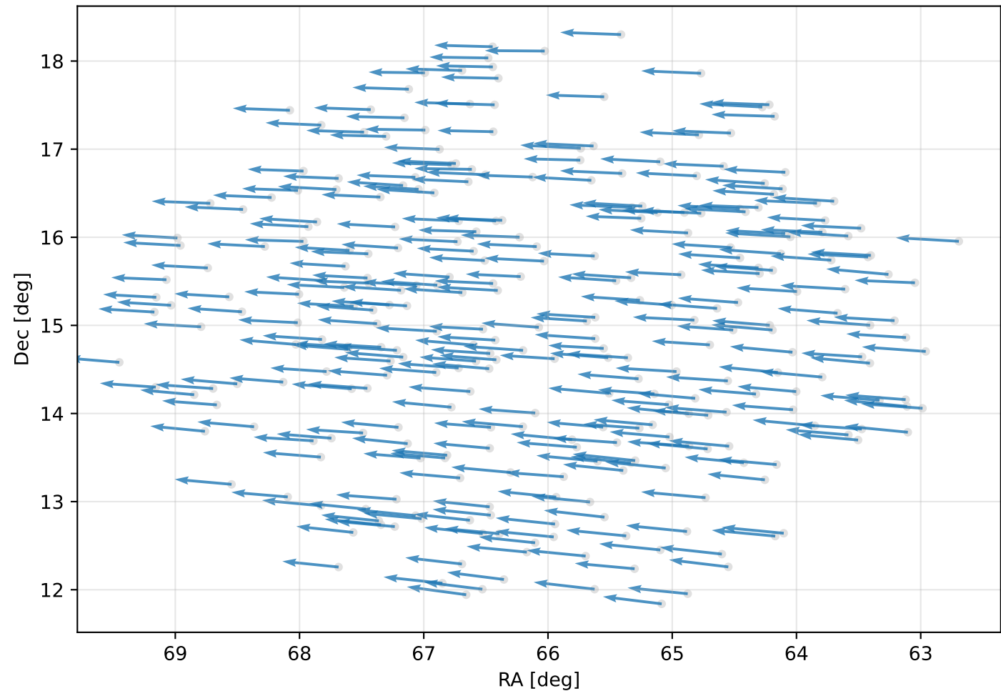
Proper-motion vector field
