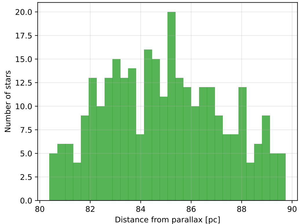
Distance distribution
