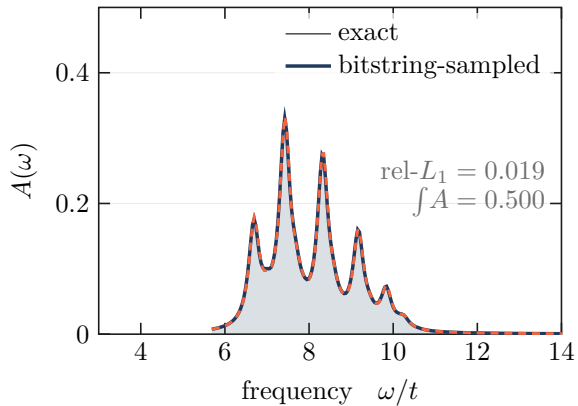
(a) bitstring reconstruction of A(\omega)
