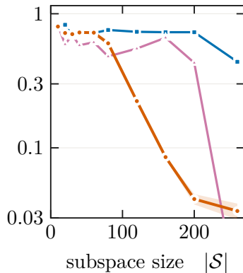
(c) U/t = 12
