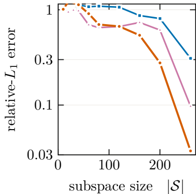
(a) U/t = 4
