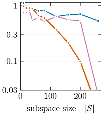
(b) U/t = 8
