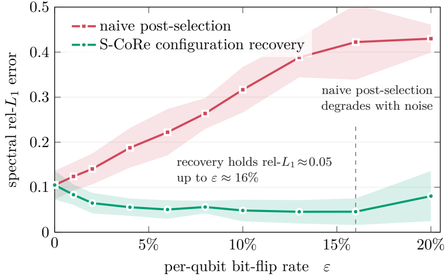
FIG. 15. Noise robustness (synthetic per-qubit bit-flip channel, L = 6 ). Spectral relative- L_1 error vs the per-qubit bit-flip rate \epsilon , applied to bitstrings Born-sampled from the exact distribution (this is a controlled classical simulation, not a device run). Naive post-selection degrades steadily, whereas S-CoRe self-consistent configuration recovery holds the error near 0.05 out to \epsilon \approx 16\% (seed-averaged over 6 seeds at 6,000 shots each; bands = \pm 1 s.d. across seeds).
