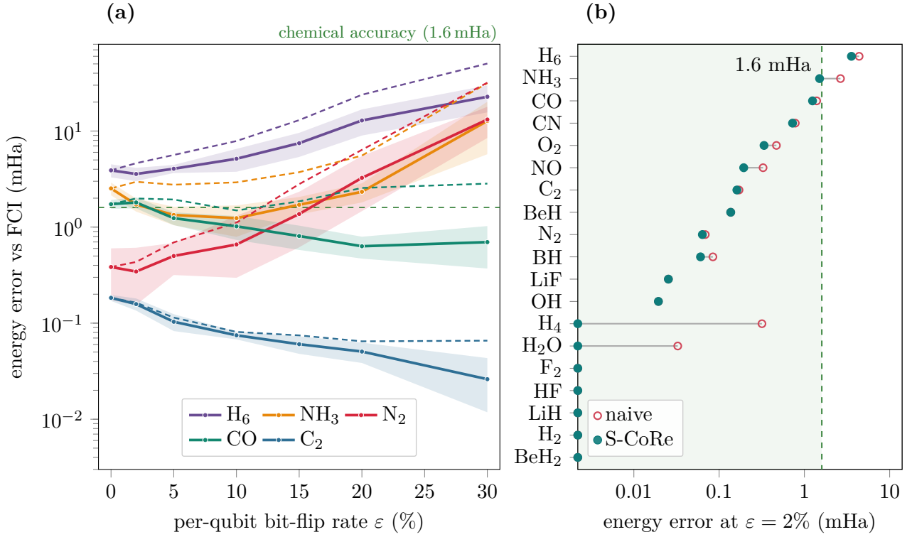
FIG. 16. SQD ground-state energy under a controlled bit-flip model across the molecular suite. (a) Energy error vs the per-qubit bit-flip rate \varepsilon for five representative molecules ( H_6 , NH_3 , N_2 , CO , C_2 ; seed-averaged over 8 seeds at 4,000 shots each, bands = \pm 1 s.d. across seeds; log scale). Solid = S-CoRe recovery, dashed = naive post-selection. The advantage of recovery over naive post-selection, both arms consuming the same corrupted bitstrings at the same rate with the same seeds, grows with noise. For CO and C_2 the error at finite \varepsilon also falls below its own \varepsilon = 0 value; that second comparison is withdrawn in Sec. IX A, because it is decided by the size of the recovered subspace, which this sweep does not record. (b) The full nineteen-molecule suite at a realistic \varepsilon = 2\% (log scale, sorted): for each molecule the naive post-selection error (open circle) is linked to the S-CoRe value (filled), so the leftward pull is the recovery gain; the shaded band is chemical accuracy ( < 1.6 mHa). Eighteen of nineteen land inside it; H_6 , the most multireference case, is the residual challenge. Panels (a) and (b) are independent seed ensembles (panel (a): 8 seeds; panel (b): 5 seeds, 4000 shots), so a given molecule's \varepsilon = 2\% value can differ by up to a factor of a few between them (for N_2 , 0.34 vs 0.06 mHa; both far below chemical accuracy).
