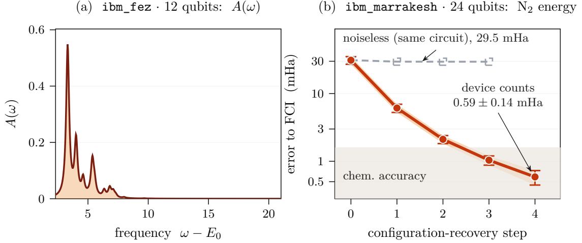
FIG. 9. The complete quantum-hardware record of this work: two runs on IBM Heron processors. (a) Electron-addition branch of the local spectral function, A_{0\uparrow}^+(\omega) , of the L = 6 periodic Hubbard ring at U/t = 4 , \eta = 0.15t (12 qubits; the classical validation of Fig. 2 is a different instance, U/t = 8 ), computed on the subspace post-selected from 350,000 computational-basis bitstrings—50,000 from each of seven circuits—measured on ibm_fez (measurement and Pauli twirling and dynamical decoupling; no readout-error mitigation and no configuration recovery). The retained shots covered the complete (N+1) sector ( |\mathcal{S}| = 300/300 ), so the reconstruction is exact by coverage; they were post-selected in reversed bit order, so every retained shot is a device error (Sec. IX A). The panel is an execution record, and neither a fidelity measurement nor a claim of advantage. (b) Ground-state energy error of stretched N_2 ( R = 2.0 Å, CAS(10e,12o)/cc-pVDZ, 24 qubits) versus self-consistent configuration-recovery step, on ibm_marrakesh (10,000 shots, CCSD-seeded local unitary cluster-Jastrow (LUCJ) circuit). Recovery on the device counts (solid) reaches 0.59 \pm 0.14 mHa of the exact FCI value—well below chemical accuracy—whereas the noiseless statevector simulation of the same circuit (dashed) is stranded at 29.5 mHa (its recorded recovery history ends at step 3, unchanged since step 2). That contrast is not read here as device noise helping : the mechanism such a reading needs is decided by the two recovered subspace sizes, and the record stores neither (Sec. IX A). The solid curve is the mean over 8 recovery seeds on the cached device counts; the shaded envelope and the capped whiskers at every step both show the \pm 1 population s.d. (normalized by 8, not 7) across those 8 seeds (widest at step 0, 31.1 \pm 4.0 mHa, where it starts together with the noiseless curve, and tapering as recovery converges to 0.59 \pm 0.14 mHa; best seed 0.40 mHa). No random-bitstring control was run, so the panel cannot separate what the device counts contributed from what recovery alone supplies; the controlled recovery-versus-no-recovery comparison, under a simulated bit-flip model, is Fig. S8. These two runs are the entirety of the quantum hardware used here; every other result in this work is an exact classical simulation.
