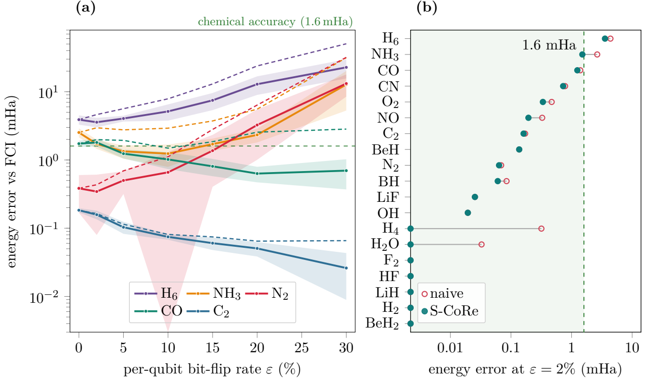
FIG. S8. SQD ground-state energy under a controlled bit-flip model across the molecular suite. (a) Energy error vs the per-qubit bit-flip rate \epsilon for five representative molecules ( H_6 , NH_3 , N_2 , CO , C_2 ; seed-averaged over 8 seeds at 4000 shots each, bands = \pm 1 s.d. across seeds, running to the bottom of the panel where the mean minus one s.d. falls below it, as for N_2 at \epsilon = 10\% ; log scale). Solid = S-CoRe recovery, dashed = naive post-selection. The advantage of recovery over naive post-selection, both arms consuming the same corrupted bitstrings at the same rate with the same seeds, grows with noise. For NH_3 , CO and C_2 the error at finite \epsilon also falls below its own \epsilon = 0 value, beyond the seed bands ( NH_3 2.53 \rightarrow 1.24 mHa at \epsilon = 10\% ); that second comparison is not used here (Sec. IX A): it is decided by the size of the recovered subspace, which this sweep does not record. (b) The full nineteen-molecule suite at a realistic \epsilon = 2\% (log scale, sorted; errors that are exact to round-off, in both arms for F_2 , HF , LiH , H_2 and BeH_2 , where the open circle is hidden behind the filled one, and after recovery for H_4 and H_2O , are drawn at the left edge of the axis): for each molecule the naive post-selection error (open circle) is linked to the S-CoRe value (filled), so the leftward pull is the recovery gain; the shaded band is chemical accuracy ( < 1.6 mHa). Eighteen of nineteen land inside it; H_6 , the most multireference case, is the residual challenge. Panels (a) and (b) are independent seed ensembles (panel (a): 8 seeds; panel (b): 5 seeds, 4000 shots), so a given molecule's \epsilon = 2\% value can differ by up to a factor of a few between them (for N_2 , 0.34 vs 0.06 mHa; both far below chemical accuracy).
