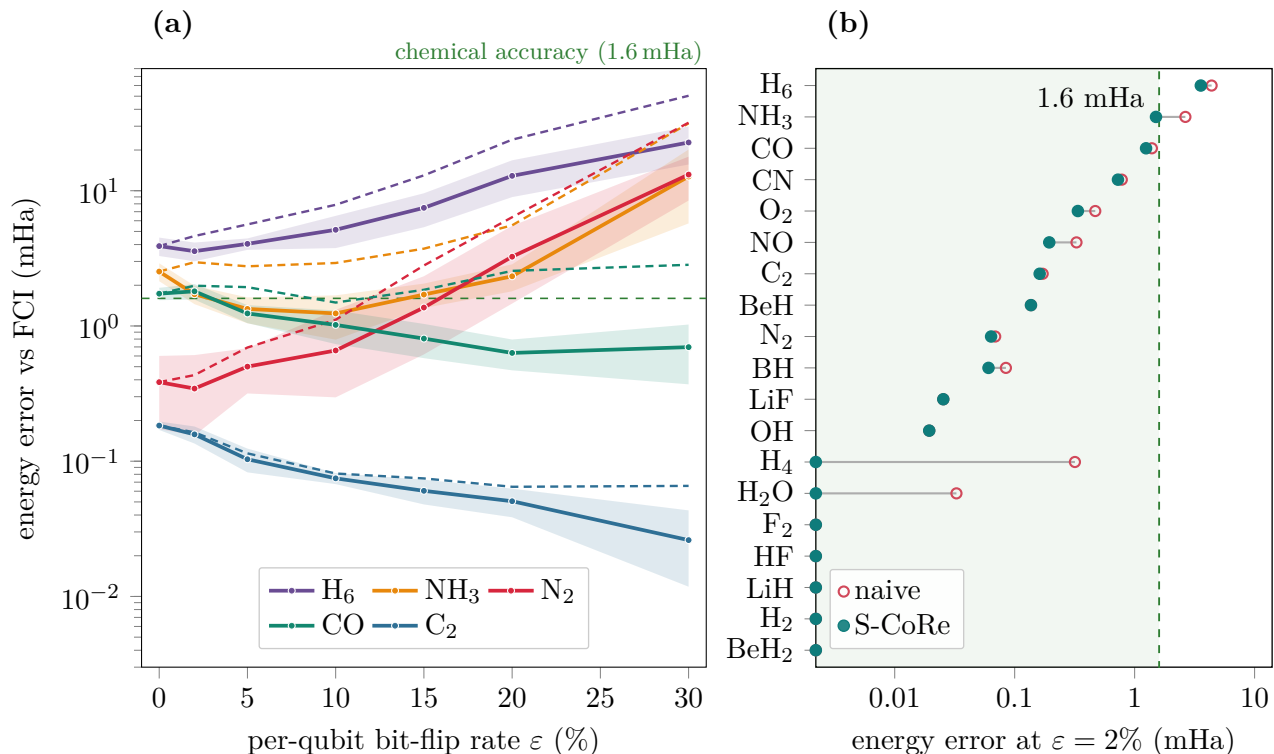
FIG. 16. SQD ground-state energy under a controlled bit-flip model across the molecular suite. (a) Energy error vs the per-qubit bit-flip rate \varepsilon for five representative molecules ( H_6 , NH_3 , N_2 , CO , C_2 ; seed-averaged over 8 seeds at 4,000 shots each, bands = \pm 1 s.d. across seeds; log scale). Solid = S-CoRe recovery, dashed = naive post-selection. The advantage of recovery over naive post-selection, both arms consuming the same corrupted bitstrings at the same rate with the same seeds, grows with noise. For CO and C_2 the error at finite \varepsilon also falls below its own \varepsilon = 0 value; that second comparison is not used here (Sec. IX A): it is decided by the size of the recovered subspace, which this sweep does not record. (b) The full nineteen-molecule suite at a realistic \varepsilon = 2\% (log scale, sorted): for each molecule the naive post-selection error (open circle) is linked to the S-CoRe value (filled), so the leftward pull is the recovery gain; the shaded band is chemical accuracy ( < 1.6 mHa). Eighteen of nineteen land inside it; H_6 , the most multireference case, is the residual challenge. Panels (a) and (b) are independent seed ensembles (panel (a): 8 seeds; panel (b): 5 seeds, 4000 shots), so a given molecule's \varepsilon = 2\% value can differ by up to a factor of a few between them (for N_2 , 0.34 vs 0.06 mHa; both far below chemical accuracy).
