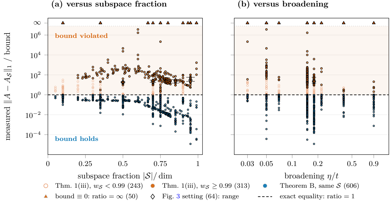
FIG. 17. The published bound of Theorem 1(iii) fails on exactly the subspaces the paper relies on; the replacement does not. For each subspace \mathcal{S} we plot the measured error \|A - A_{\mathcal{S}}\|_1 divided by the bound, so every point above the dashed line at 1 is a violation. Orange: the published weight bound 2\|\varphi\|^2(1 - w_{\mathcal{S}}) , split by captured weight (filled, w_{\mathcal{S}} \geq 0.99 ; open, w_{\mathcal{S}} < 0.99 ). Blue: Theorem B as stated, \min\{\|\varphi\|^2(1 + w_{\mathcal{S}}), (\|\varphi\| + \|\varphi_{\mathcal{Q}}\|)(\|\varphi_{\mathcal{Q}}\| + \Lambda_{\mathcal{S}}(\eta)/\eta)\} , on the same subspaces. We pooled 621 subspaces from five machine-readable sweeps written by two independent implementations (239 + 4 from the original sweep; 162 + 112 + 104 from an independent re-implementation); 15 of them reproduce the target to within double-precision round-off (relative L_1 \leq 10^{-10} ) and define no ratio, leaving 606 live subspaces, of which 156 are finite-shot realisations at 4000 shots per snapshot and the remainder are deterministic weight-ordered or structured selections. The published bound is violated on 468 of the 606. On 50 of them it is identically zero: those subspaces carry the whole weight to double precision ( w_{\mathcal{S}} = 1 exactly, and K_{\mathcal{S}} \in \{0, 1, 2\} , so the remaining term is the undefined constant C\rho^{-K_{\mathcal{S}}} ); their ratio is infinite and they are drawn on the row marked \infty , above the dotted rule. Among the 313 finite-ratio points with w_{\mathcal{S}} \geq 0.99 —the regime the paper invokes— every one is a violation, the mildest by a factor 2.10; with the 50 infinite ones that is 363 of 363, and the finite factors reach 3.66 \times 10^6 . Below w_{\mathcal{S}} = 0.99 the bound survives on 138 of 243 points, but only where the relative error is already of order unity, so it excludes nothing there. Diamonds mark the configuration of Fig. 3 ( L = 8 , U/t = 8 , \eta = 0.18t , momentum seeds c_{k\uparrow}^\dagger|\Psi_0\rangle , subspace fractions 0.50/0.70/0.85/0.95, both branches, eight momenta): that reconstruction reproduces the deposited sampled_akw_L8.json to 2.1 \times 10^{-8} per momentum, and its violation factor is 15.1–57.3, of which 15.1–33.7 at the published fraction 0.85. Those 64 rows sit at only four abscissae, so they are drawn as a min–median–max whisker at each one rather than as 64 overlapping markers (medians 18.5, 23.6, 26.5, 29.9 at fractions 0.50, 0.70, 0.85, 0.95); each of them is also plotted individually inside the filled orange series, which is where their scatter can be read. Theorem B is violated on none of the 606; its ratios span 1.18 \times 10^{-5} to 0.9999999997. That maximum is reached on four subspaces with w_{\mathcal{S}} = 0 exactly, where A_{\mathcal{S}} \equiv 0 and \|A - A_{\mathcal{S}}\|_1 = \|\varphi\|^2 equals the trivial cap by algebra—the branch that carries no information—and the leakage branch \Lambda_{\mathcal{S}}(\eta)/\eta is the smaller of the two on only 61 of the 606 rows: the figure shows that Theorem B holds , not that it is tight. In (b) the \eta axis is not a sweep within one model: the Hubbard-chain rows exist only at \eta/t = 0.05, 0.15, 0.18 and the stress families (XXZ, t -V, Anderson, sparse random) only at 0.03, 0.07, 0.22, 0.40, 0.90, so no trend across the full axis may be read from it.
