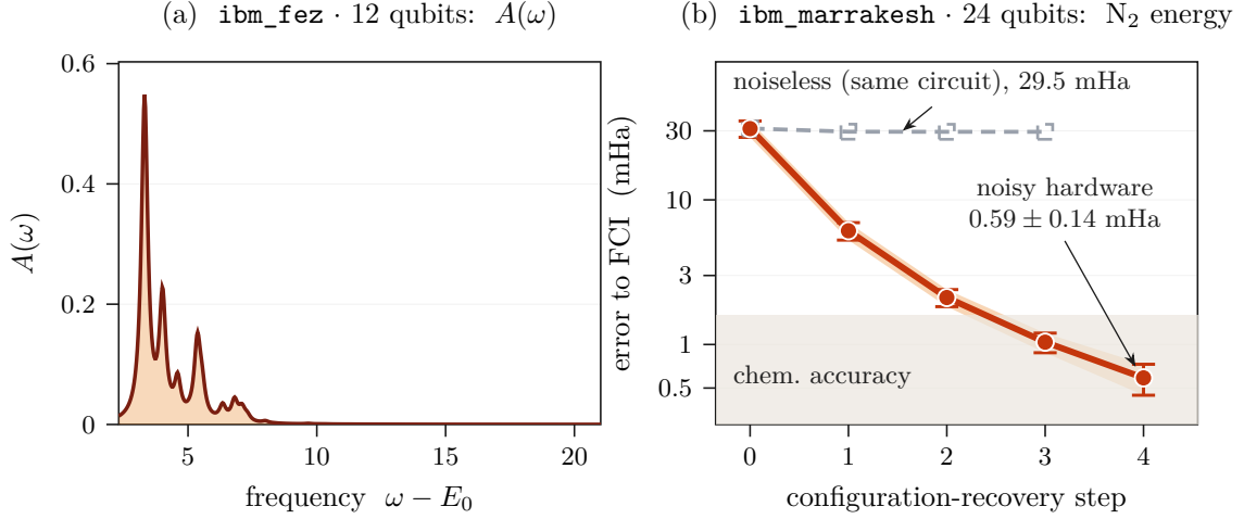
FIG. 14. The complete quantum-hardware record of this work: two runs on IBM Heron processors. (a) Single-particle spectral function A(\omega) of the L = 6 Hubbard model at U/t = 4 , \eta = 0.15t (12 qubits); the classical validation of Fig. 2 is a different instance, U/t = 8 , reconstructed from 350,000 computational-basis bitstrings—50,000 from each of seven circuits—sampled on ibm_fez (TREX readout twirling, Pauli twirling, and dynamical decoupling). The device histogram covered the complete (N+1) sector ( |S| = 300/300 ), so the reconstruction is exact by coverage—a proof of principle, and neither a fidelity measurement nor a claim of advantage. (b) Ground-state energy error of stretched N_2 ( R = 2.0 Å, CAS(10e,12o)/cc-pVDZ, 24 qubits) versus self-consistent configuration-recovery step, on ibm_marrakesh (10,000 shots, double-factorized Trotter circuit). The noisy device (solid) reaches 0.59 \pm 0.14 mHa of the exact FCI value—well below chemical accuracy—whereas the noiseless statevector simulation of the same shallow circuit (dashed) is stranded at 29.5 mHa. That contrast is not read here as device noise helping : the mechanism such a reading needs is decided by the two recovered subspace sizes, and the record stores neither (Sec. IX A). The solid curve is the mean over 8 recovery seeds on the cached device counts; the shaded envelope and the capped whiskers at every step both show the \pm 1 s.d. spread across those 8 seeds (widest at step 0, 31.1 \pm 4.0 mHa, where it starts together with the noiseless curve, and tapering as recovery converges to 0.59 \pm 0.14 mHa; best seed 0.40 mHa). The systematic version across nineteen molecules under a controlled noise model is Fig. 16. These two runs are the entirety of the quantum hardware used here; every other result in this work is an exact classical simulation.
