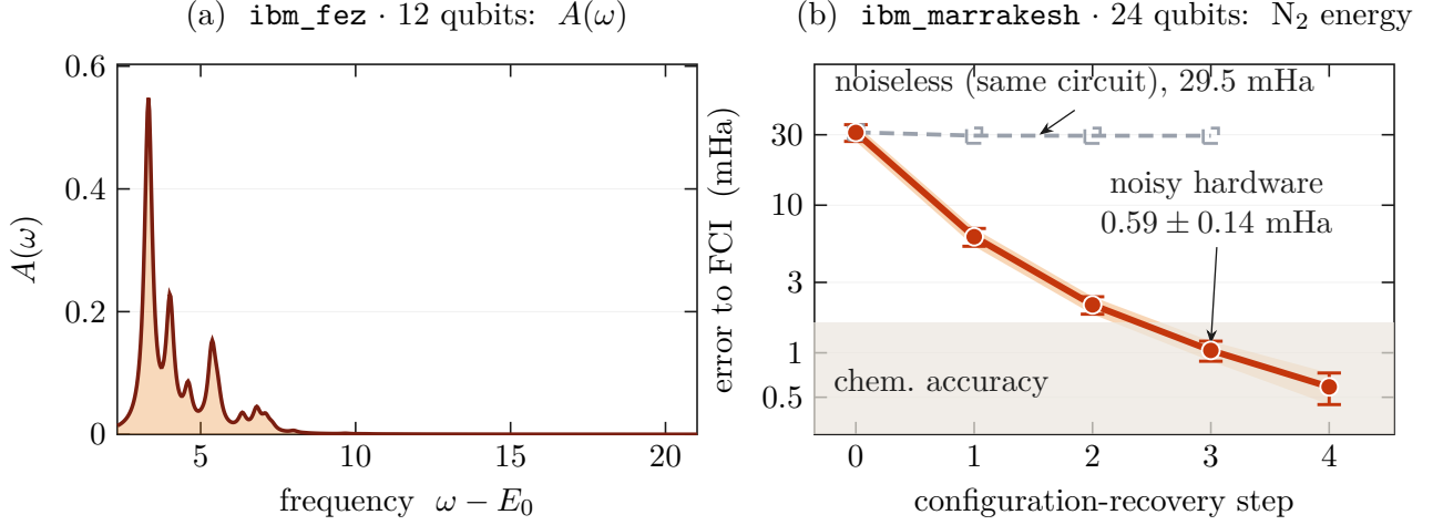
Figure 15. The complete quantum-hardware record of this work: two runs on IBM Heron processors. (a) Single-particle spectral function A(\omega) of the L = 6 Hubbard model at U/t = 4 , \eta = 0.15 t (12 qubits; the classical validation of Fig. 3 is a different instance, U/t = 8 ), reconstructed from 50,000 computational-basis bitstrings sampled on ibm_fez (TREX readout twirling, Pauli twirling, and dynamical decoupling). The device histogram covered the complete (N+1) sector ( |\mathcal{S}| = 300/300 ), so the reconstruction is exact by coverage—a proof of principle, not a fidelity or beyond-classical claim. (b) Ground-state energy error of stretched N_2 ( R = 2.0 Å, CAS(10e,12o)/cc-pVDZ, 24 qubits) versus self-consistent configuration-recovery step, on ibm_marrakesh (10,000 shots, double-factorized Trotter circuit). The noisy device (solid) reaches 0.59 \pm 0.14 mHa of the exact FCI value—well below chemical accuracy—whereas the noiseless statevector simulation of the same shallow circuit (dashed) is stranded at 29.5 mHa: device noise, filtered through configuration recovery, populates valid configurations the ideal shallow circuit misses. The solid curve is the mean over 8 recovery seeds on the cached device counts; the shaded envelope and the capped whiskers at every step both show the \pm 1 s.d. spread across those 8 seeds (widest at step 0, 31.1 \pm 4.0 mHa, where it starts together with the noiseless curve, and tapering as recovery converges to 0.59 \pm 0.14 mHa; best seed 0.40 mHa). The systematic version across nineteen molecules under a controlled noise model is Fig. 17. These two runs are the entirety of the quantum hardware used here; every other result in this work is an exact classical simulation.
