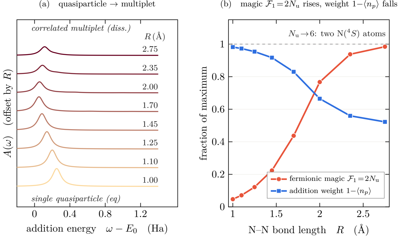
FIG. S6. Magic and multireference character in N_2 dissociation. (a) The exact addition spectral function A(\omega) (orbital-projected, CAS(6,6), cc-pVDZ) along the triple-bond stretch, offset vertically, one row per R : the sharp coherent quasiparticle peak near equilibrium ( R = 1.0 Å, slightly compressed from the R_{\text{eq}} = 1.098 Å of Table S10) broadens into a correlated multiplet on dissociation as its spectral weight collapses. (b) Two physically independent quantities along the same coordinate. The fermionic magic obeys the exact identity \mathcal{F}_1 = 2N_u [Eq. (17), verified to < 10^{-13} ], so a single curve carries both: it rises with the orbital-rotation-invariant multireference count—the effective number of unpaired electrons N_u = \sum_i n_i(2 - n_i) from the natural-orbital occupations n_i , approaching its atomic limit of 6 (the two triplet N(^4S) atoms) as the bond fully breaks. The integrated addition weight \int A^+ d\omega = 1 - \langle \hat{n}_p \rangle (from panel a) falls from 0.98 to 0.52 over the same stretch; the two cross as the bond breaks. The active-space CASCI energies are converged to 1.1 \times 10^{-13} Ha, which is a convergence check and not a validation against an independent method (Sec. S15.1).
