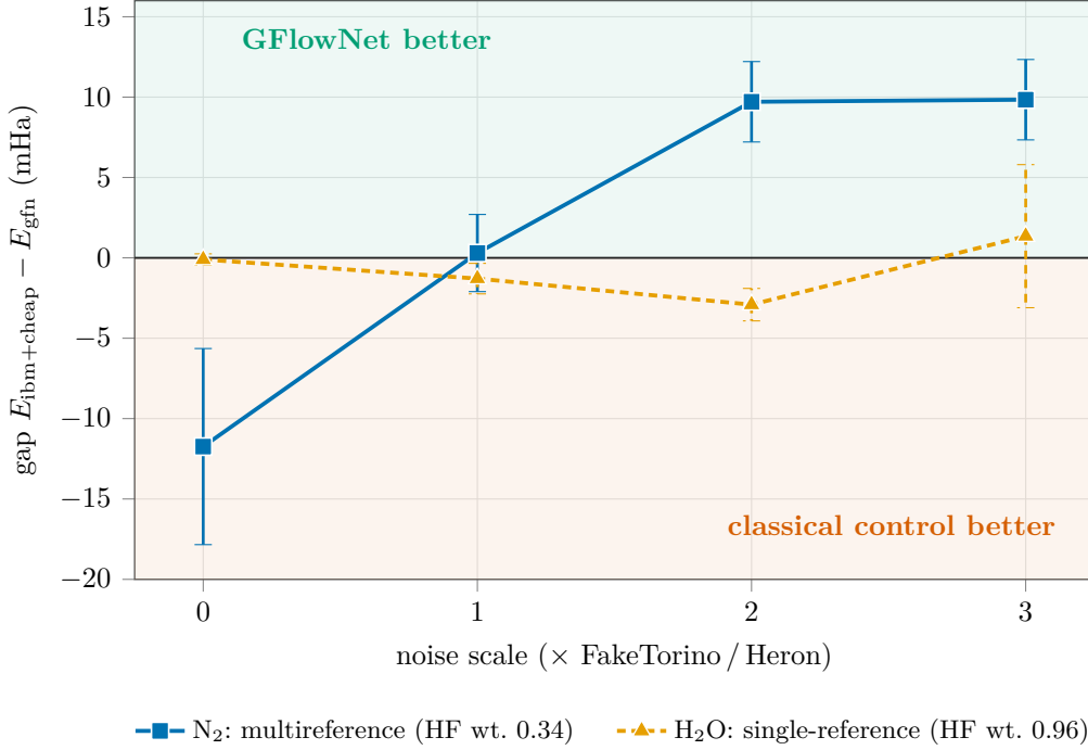
Figure 10. The noise crossover is specific to the multireference regime (two FCI-verifiable systems). Energy-error gap between the fair classical control (S-CORE recovery + cheap-prior fill) and the fused generative proposer, vs simulated device-noise scale (FakeTorino / Heron r1), as mean \pm s.d. over five seeds. Strongly multireference stretched N 2 (blue; Hartree–Fock weight 0.34) shows the crossover: the classical control is better or tied at low noise ( -11.7 \pm 6.1 at 0\times , 0.3 \pm 2.4 mHa at 1\times ) and the constraint-respecting generative proposer pulls ahead only at higher noise ( 9.7 \pm 2.5 and 9.8 \pm 2.5 mHa at 2\times and 3\times ; paired t_4=8.7 , p\approx 0.001 , Gaussian-equivalent \sim 3.3\sigma — not the naïve 9.7/\text{s.d.} effect size). Single-reference H 2 O (orange; HF weight 0.96) shows no crossover: the classical control wins or ties throughout, and is in fact significantly better at 2\times ( -2.9 \pm 1.0 mHa, paired t_4=-6.4 ), even though H 2 O suffers the same valid-shot starvation (53% of shots lost at 3\times , versus 51% for N 2 ). The contrast isolates the mechanism: valid-shot starvation alone does not produce a generative advantage; the crossover requires both noise and an intrinsically imperfect cheap prior, i.e. multireference character (§7). A conditional, regime-dependent effect at energies above chemical accuracy — not a universal win.
