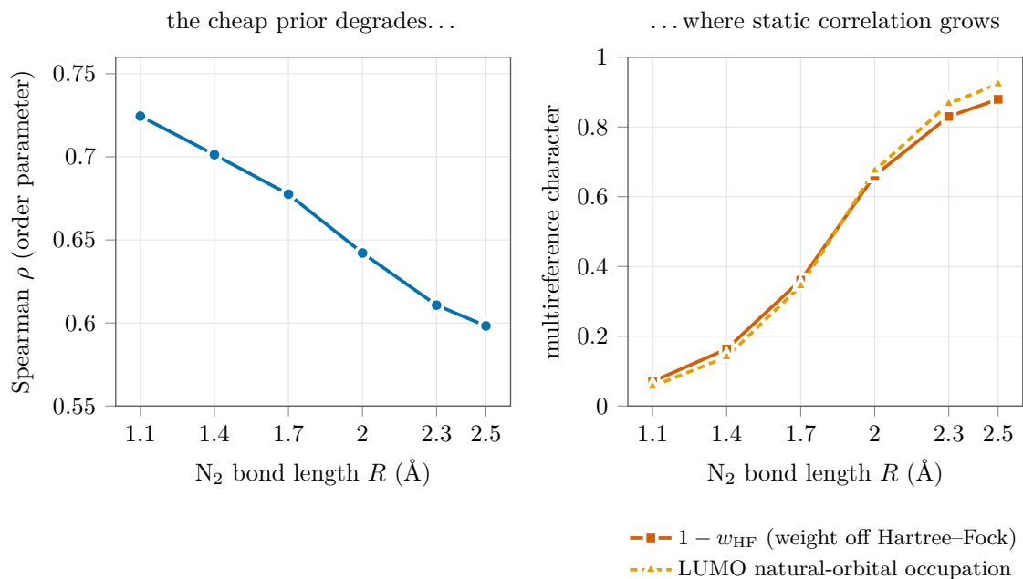
Figure 9. The order parameter, measured on N_2 across geometries. (a) The Spearman rank correlation between the cheap Epstein–Nesbet reward and the exact FCI |c|^2 (over all 792 \alpha -strings) falls monotonically as the triple bond stretches, from \rho=0.72 near equilibrium to 0.60 at R=2.5 Å. (b) Over the same interval the wavefunction becomes strongly multireference: the weight carried by determinants other than Hartree–Fock rises from 0.07 to 0.88, and the frontier natural-orbital occupations open from the closed-shell 2/0 toward the dissociation limit 1/1 (LUMO occupation 0.06 \rightarrow 0.92). The cheap classical importance signal that makes an SQD subspace verifiable degrades exactly where static correlation makes it hard to construct — so the single scalar \rho predicts, before any hardware is run, where a learned or quantum proposer has room to help.
