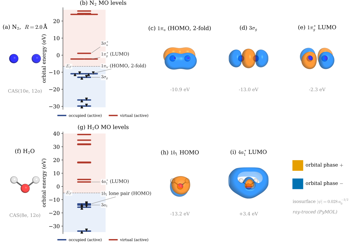
Figure 2. The molecular systems, their active-space orbital-energy structure, and the frontier orbitals. (a,f) Ray-traced ball-and-stick geometries of stretched N_2 ( R = 2.0 \text{ \AA} , CAS(10e,12o)) and H_2O ( r_{OH} = 1.24 \text{ \AA} , \angle HOH = 104.4^\circ , CAS(8e,12o) — also stretched, by 29% against its 0.958 \text{ \AA} equilibrium, but far less so than N_2 and still dominated by its Hartree-Fock reference). (b,g) Molecular-orbital energy-level diagrams (restricted Hartree-Fock, eV): occupied active levels (blue) carry their two electrons as up/down arrows, virtual active levels are red, the shaded band is the complete active space, and E_F marks the HOMO-LUMO midpoint; the deep 1s core is frozen and off-scale. (c-e) Ray-traced (PyMOL) isosurfaces of the N_2 frontier orbitals — the two-fold-degenerate 1\pi_u HOMO (-10.9 eV; note the axis-containing nodal plane of \pi symmetry), the non-degenerate 3\sigma_g level just below it (-13.0 eV; cylindrically symmetric about the bond axis), and the 1\pi_g^* LUMO (-2.3 eV) — with their RHF energies. The crowding of these frontier levels as the triple bond stretches, and the collapse of the bonding-antibonding gaps ( 1\pi_u/1\pi_g^* , 3\sigma_g/3\sigma_u^* ) toward dissociation, is what makes stretched N_2 strongly multireference: at R = 2.0 \text{ \AA} the FCI natural-orbital occupations of the frontier pair are already 1.32/0.67 (versus the closed-shell 2/0) and the Hartree-Fock determinant carries only 34% of the exact weight (§7). (h,i) The H_2O 1b_1 lone-pair HOMO and 4a_1^* LUMO. Isosurfaces at |\psi| = 0.028 a_0^{-3/2} ; orbital phases orange/blue.
