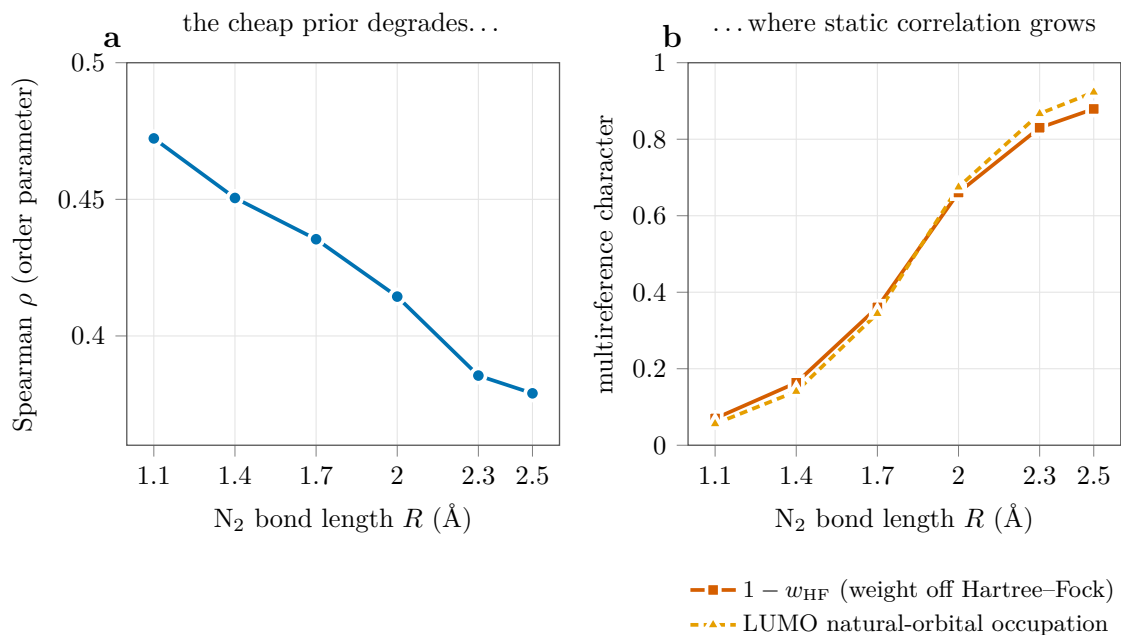
Figure 9. The cheap prior degrades with multireference character (N 2 across geometries). (a) The Spearman rank correlation between the cheap Epstein–Nesbet reward and the exact FCI |c|^2 (over all 792 \alpha -strings) falls monotonically as the triple bond stretches, from \rho=0.47 near equilibrium to 0.38 at R=2.5 Å (symmetry-adapted gauge; see the header of orderparam.dat for the thresholding convention). (b) Over the same interval the wavefunction becomes strongly multireference: the weight carried by determinants other than Hartree–Fock rises from 0.07 to 0.88, and the frontier natural-orbital occupations open from the closed-shell 2/0 toward the dissociation limit 1/1 (LUMO occupation 0.06 \rightarrow 0.92). The cheap classical importance signal that makes an SQD subspace verifiable degrades exactly where static correlation makes it harder to construct — so we propose the single scalar \rho as a low-cost coordinate , computable system by system before any hardware is run, for where a learned or quantum proposer might have room to help. Whether it in fact predicts that is the open test set out in §7, not a result of this figure.
