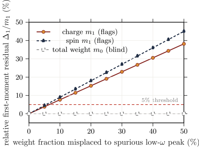
FIG. 6. The moment test applied to the collective (charge and spin) channels. The same reconstruction-independent screen of Fig. ??, applied without modification to the charge S(q, \omega) and spin S^{zz}(q, \omega) structure factors of Fig. ?? (whose spectra are shown there). For each channel a wrong reconstruction misplaces band weight into a spurious low-frequency phantom peak—in-gap ( \omega = 2.0t ) for the gapped charge channel, near-zero ( \omega = 0.10t ) for the gapless spin channel—conserving the total weight m_0 exactly. At q/\pi = 2/3 the total-weight sum rule m_0 (grey) stays blind for both channels, while the reconstruction-independent first moment m_1 = \frac{1}{2}\langle [A^\dagger, [H, A]] \rangle rises through the falsification threshold for both the charge ( \rho_q = \sum_j e^{-iqj} n_j , oxblood) and spin ( S_q^z = \sum_j e^{-iqj} S_j^z , indigo) probes. The operator moments reproduce the exact Lehmann moments to \sim 10^{-15} at every momentum q/\pi \in \{1/3, 2/3, 1\} . Hubbard ring L = 6 , U/t = 8 , PBC, half filling; exact simulation.
