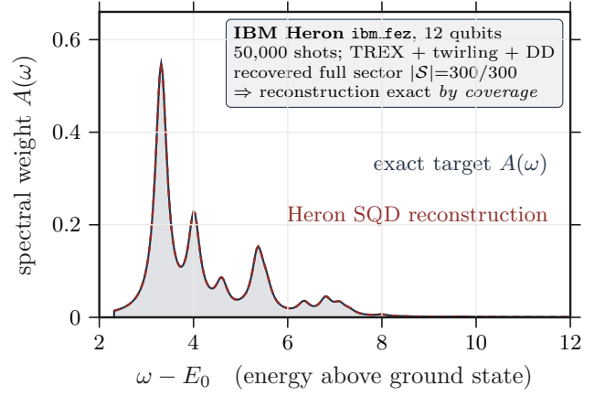
FIG. 11. Executability precursor ( L = 6 , full-sector recovery) . An earlier full-coverage run establishing only that the pipeline executes on hardware; the graded coverage test that actually exercises the falsifier from retained counts is Fig. ?? . At the demonstrated size— L = 6 Hubbard, U/t = 4 , N+1 electron-addition sector ( 4 \uparrow, 3 \downarrow )—a real IBM Heron run ( ibm_fez , 12 qubits, 50,000 shots, TREX + Pauli twirling + dynamical decoupling) recovered the full determinant sector ( |S| = 300/300 ), so the sample-based-diagonalization reconstruction coincides with exact diagonalization by coverage (it lies on the exact curve). The run establishes hardware executability and full-sector recovery, not a device-error line shape or a fidelity claim [? ? ].
