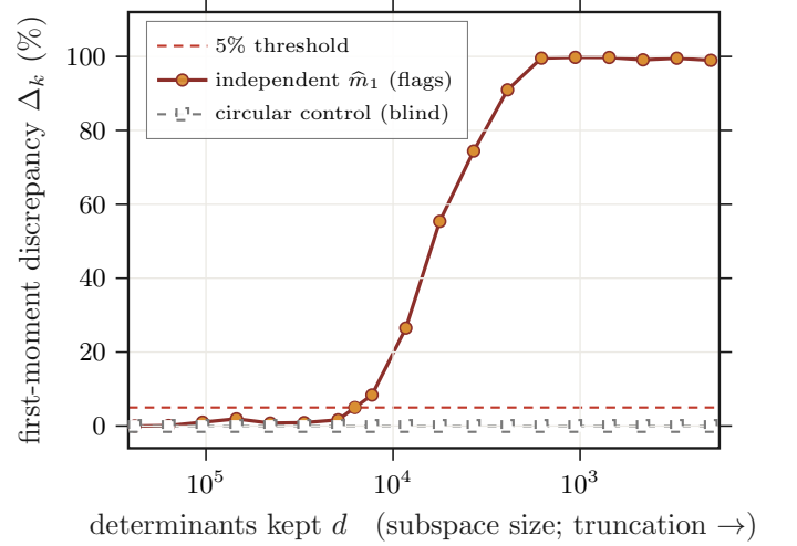
FIG. 7. Independent vs. back-computed moment discrepancy under determinant-subspace truncation. The determinant subspace of the doped L = 12 Hubbard ring is truncated to its top d configurations by |\psi_0|^2 (the sample-based-diagonalization ordering; full support n_{\text{sup}} = 2.4 \times 10^5 ), and the current first moment is recomputed within it. On this truncated data the reconstruction- independent ground-state estimator’s discrepancy \Delta_1^{\text{rel}} = |\hat{m}_1 - \tilde{m}_1|/\hat{m}_1 stays negligible while the subspace is large but grows sharply once truncation becomes severe, crossing the falsification threshold at d \approx 1.6 \times 10^4 and saturating near 100%; a back-computed (circular) control read off the reconstructed spectrum stays identically zero and reports it consistent. The independent estimator therefore discriminates the subspace-truncation error class; the first moment stays robust until the subspace is small, so the screen catches severe truncation rather than mild undersampling. The circular control is blind by construction [? ? ?]. Sector-basis Lanczos: the truncated first moment is \langle J\psi_0^d | (H_d - E_0^d) | J\psi_0^d \rangle from one subspace ground state, no full diagonalization [? ?].
