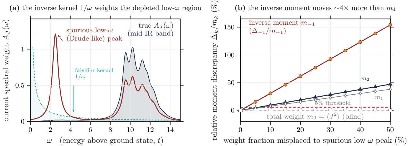
FIG. 5. The current-response test: a wrong distribution of correct total weight. Doped one-dimensional Hubbard ring ( L = 12 , U/t = 8 , filling 2/3 , periodic boundaries; optical conductivity \text{Re } \sigma \propto A_J/\omega ). A wrong reconstruction moves a fraction f of the weight above 6t into a spurious pole at 2.5t (a Drude-like peak), keeping m_0 = \langle J^2 \rangle fixed. (a) The true regular spectrum (indigo) is a mid-infrared/Mott band with only 1.4% of m_0 below 6t ; the spurious peak (oxblood) sits where the kernel 1/\omega (teal) is large. (b) Relative discrepancies \Delta_k/m_k against f , with every moment evaluated exactly on the ground state. The total weight is unchanged ( \Delta_0/m_0 < 10^{-13} ); m_1 = \frac{1}{2}\langle [J, [H, J]] \rangle moves by up to 38%, m_2 by up to 47%, and m_{-1} = \frac{1}{2}\langle -\hat{T} \rangle - D = 0.324 by up to 154%. The 5% line is a common relative reference, not the deployed threshold. Under the deployed rule (2% bias budget, N_s = 5 \times 10^4 ) the thresholds are 4.3% of m_1 and of m_2 but 61% of m_{-1} , because m_{-1} is a 94% cancellation between \frac{1}{2}\langle -\hat{T} \rangle and the Kohn stiffness D ; m_2 then rejects first ( f \approx 0.046 ), m_1 next (0.057) and m_{-1} last (0.20). D is obtained from the flux curvature, not from the same samples. The identity for m_{-1} is verified against the Lehmann sum over the computed poles to a relative 2 \times 10^{-15} on open chains of L = 6 and 8 , 2 \times 10^{-14} on the open L = 12 chain and, with the stiffness correction, 2 \times 10^{-6} on this ring. Sector-basis Lanczos ground state with Haydock/Ritz current poles [36, 37, 73, 75].
