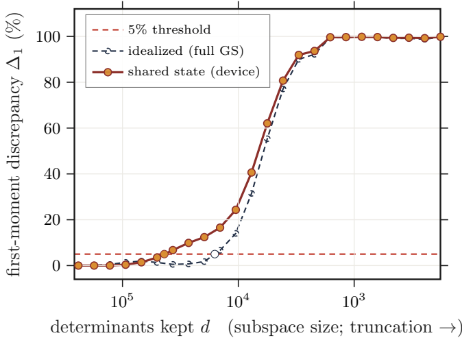
FIG. 8. Shared-state discrimination: the operator leak on a single subspace state. Both first-moment branches are evaluated on the same subspace ground state |0_S\rangle of H_S = \Pi_S H \Pi_S , with shared reference e_0 = \langle 0_S | H | 0_S \rangle , using only what a sample-based-diagonalization pipeline has (Appendix B); the evaluation is classical. Solid (oxblood, amber band): the shared-state discrepancy \Delta_1^{\text{shared}} = |\hat{m}_1 - \bar{m}_1|/\hat{m}_1 , with \hat{m}_1 = \langle 0_S | J(H - e_0)J | 0_S \rangle formed with the full operators (reaching determinants outside \mathcal{S} ) and \bar{m}_1 = \int \omega A(\omega) d\omega the within- \mathcal{S} reconstruction moment; their difference is the k=1 operator leak of Eq. (B3). Dashed (indigo): the idealized curve of Fig. 7, with \hat{m}_1 evaluated on the exact full-sector ground state. As the retained determinant count d falls (truncation \rightarrow ), the shared-state discrepancy rises by about five orders of magnitude (non-monotone near both ends: below 10^{-4} near full support, and at saturation) and crosses the illustrative 5% threshold at d \approx 4.4 \times 10^4 (18% coverage). The idealized curve crosses at d \approx 1.6 \times 10^4 (7%), after an accidental dip near d \sim 4 \times 10^4 where the full-state reference and the truncated reconstruction track each other. Both saturate near 100%. L = 12 doped Hubbard ring ( N_\uparrow = N_\downarrow = 4 , 2/3 filling), U/t = 8 , sector-basis Lanczos.
