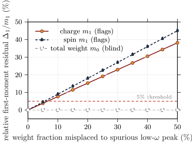
FIG. 6. The moment test on the collective (charge and spin) channels. The screen of Fig. 5, applied without change to the charge S(q, \omega) and spin S^{zz}(q, \omega) structure factors of a half-filled Hubbard ring ( L = 6 , U/t = 8 , periodic boundaries; exact simulation). For each channel a wrong reconstruction moves band weight into a spurious low-frequency peak—in the gap ( \omega = 2.0t ) for the gapped charge channel, near zero ( \omega = 0.10t ) for the gapless spin channel—conserving the total weight m_0 exactly. At q/\pi = 2/3 the total weight m_0 (grey) stays blind for both channels, while the relative first-moment residual of the charge ( \rho_q = \sum_j e^{-iqj} n_j , oxblood) and spin ( S_q^z = \sum_j e^{-iqj} S_j^z , indigo) probes grows linearly and crosses a fixed 5% relative threshold, a guide rather than the deployed rule \tau_1 . The operator moments reproduce the exact Lehmann moments to better than 10^{-14} at every momentum q/\pi \in \{1/3, 2/3, 1\} . The L = 12 spectra of the same channels are shown in Fig. 4.
