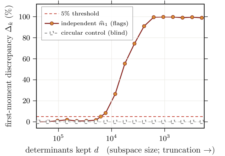
FIG. 7. Independent vs. back-computed moment discrepancy under determinant-subspace truncation (idealized estimator). The determinant subspace of the doped L = 12 Hubbard ring ( N_\uparrow = N_\downarrow = 4 , U/t = 8 ) is truncated to its top d configurations by |\psi_0|^2 (the sample-based-diagonalization ordering; full support n_{\text{sup}} = 2.4 \times 10^5 ), and the current first moment is recomputed within it. The reconstruction-independent discrepancy \Delta_1^{\text{rel}} = |\hat{m}_1 - \bar{m}_1|/\hat{m}_1 , with \hat{m}_1 evaluated on the exact full-sector ground state, stays below 2% down to 8% coverage. It then grows sharply, crosses an illustrative fixed 5% threshold at d \approx 1.6 \times 10^4 (7% coverage) and saturates near 100%. The back-computed (circular) control compares \bar{m}_1 with itself and is zero by definition [15, 16]. The screen catches severe truncation, not mild undersampling. Figure 8 removes the full-sector idealization. Sector-basis Lanczos: the truncated first moment is \langle J\psi_0^d | (H_d - E_0^d) | J\psi_0^d \rangle from one subspace ground state, with no full diagonalization [73].
