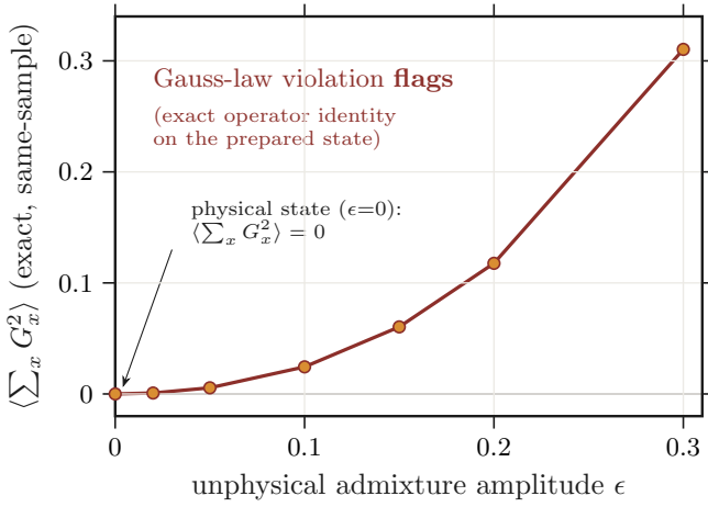
FIG. 15. A state-level check: the Gauss-law identity. In the U(1) lattice Schwinger model every G_x annihilates physical states, so they have \langle \sum_x G_x^2 \rangle = 0 ; [H, G_x] = 0 keeps the dynamics in that sector. The plotted state is |\psi(\epsilon)\rangle \propto (1 - \epsilon)|\psi_0\rangle + \epsilon|\phi_u\rangle , with |\psi_0\rangle the physical ground state and |\phi_u\rangle the lowest-energy charge-neutral state with the smallest violation, \sum_x G_x^2 = 2 . Here \epsilon is an amplitude: the unphysical weight is f_u = \epsilon^2 / [(1 - \epsilon)^2 + \epsilon^2] , only 0.155 at \epsilon = 0.3 , and the curve equals 2f_u by construction. It is computed exactly on the state vector; no sampling is simulated. The check tests the prepared state, not a reconstructed spectrum, and targets gauge-symmetry breaking, an error class the moment test does not address. N = 4 staggered sites, 3 spin- \frac{1}{2} links, open boundaries, w = 1 , m = 0.6 ; generator src/export_gauss_state.py (see text).
