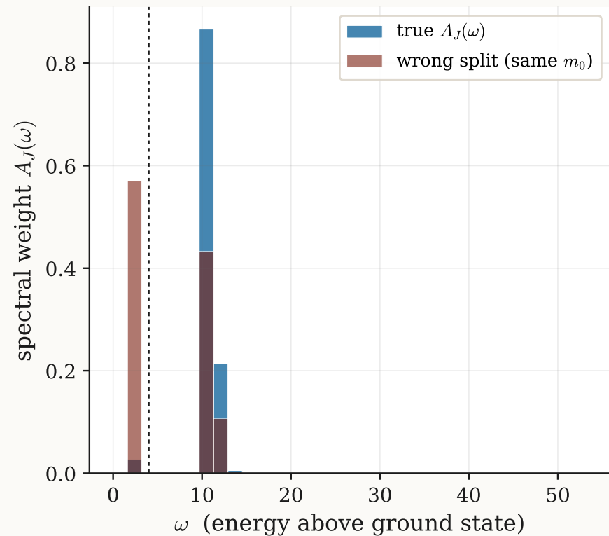
A wrong split that passes the f -sum
