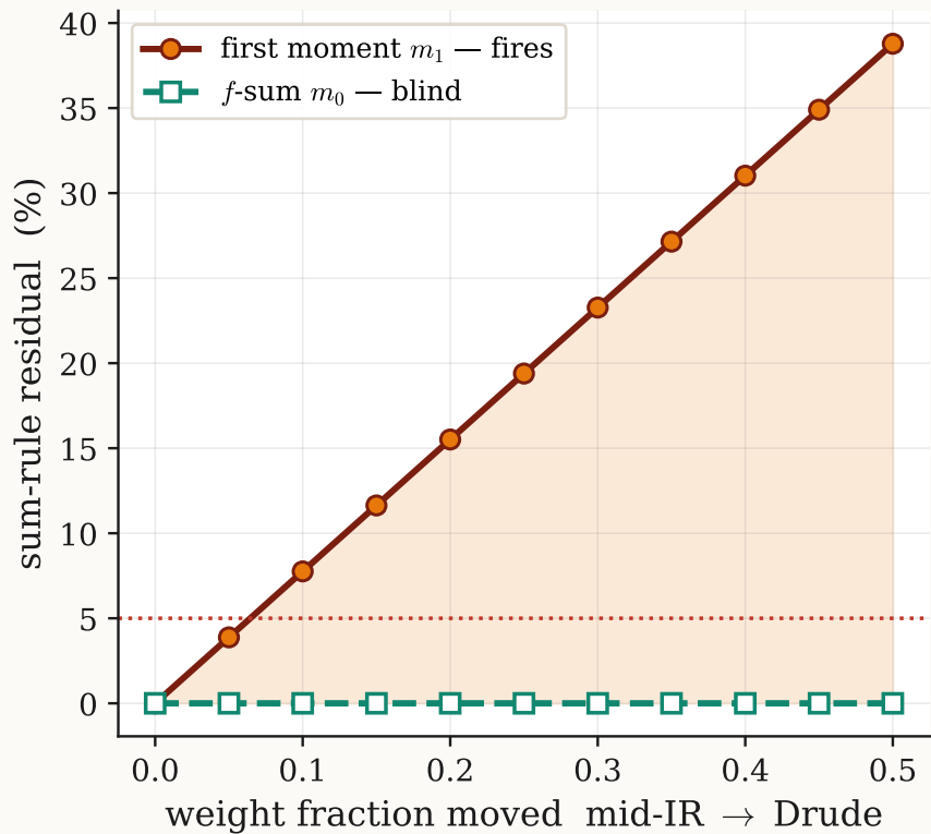
The first moment falsifies what the f -sum misses
