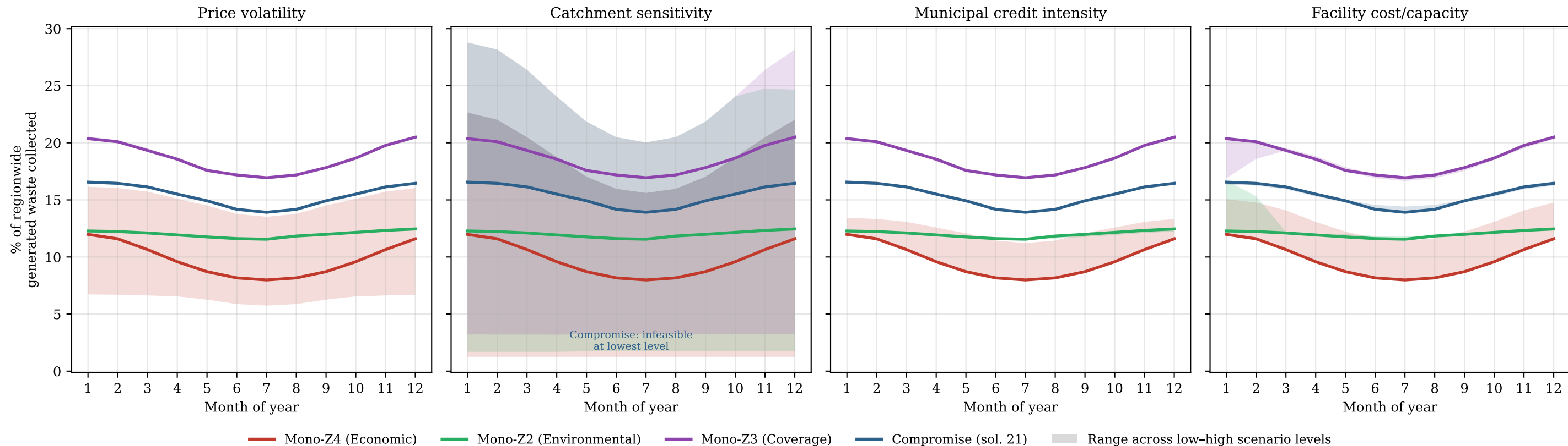
Monthly collection coverage vs. true regionwide waste generation (solid line = base level; shaded band = range across the OFAT scenario)
