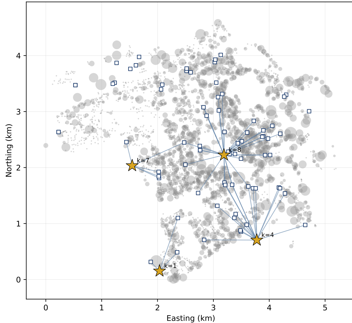
Best Reliable (gap-wise) Economic Solution Z_1=197,892\text{€} , 4 facilities, gap=5.7%
